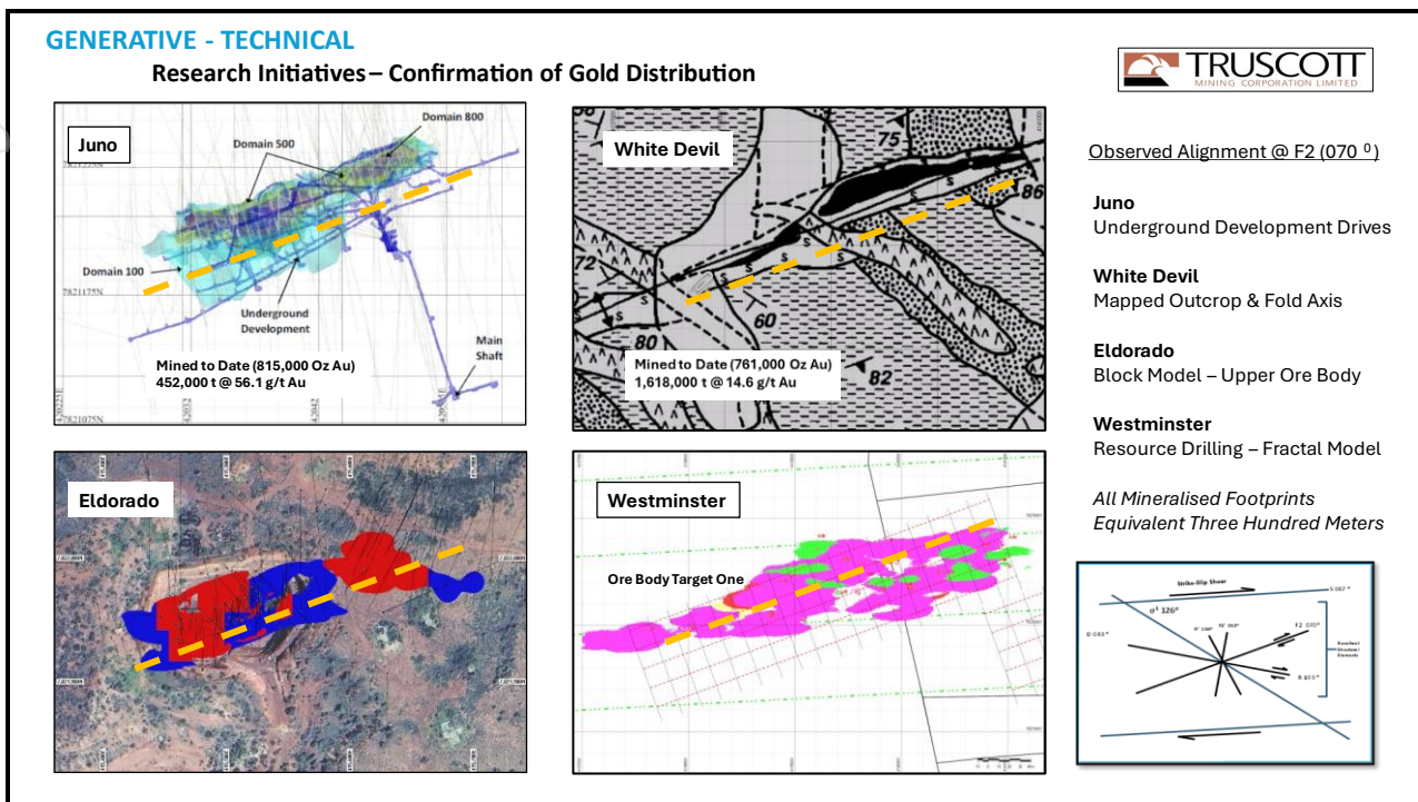
Figure Nine: Mineral Accumulations @ Fractal Four Dilation – Alignment with F2 (070°) Fold Elements
