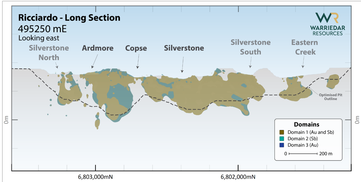
Figure 8: Sb mineralisation shell used for the MRE (Domain 1 and Domain 2).
