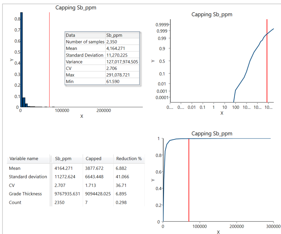
Figure 7: Capping analysis for Sb grade shell.
