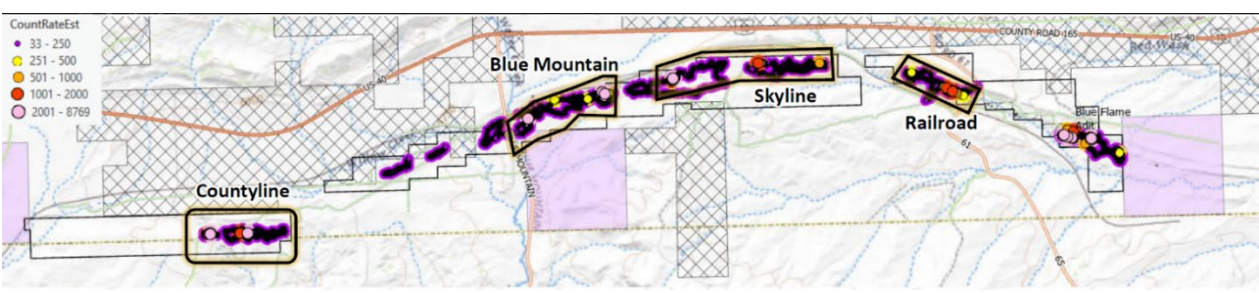
Figure 3: Prospect location map highlighting identified radiometric anomalies across the four main exploration targets: County Line, Blue Mountain, Skyline, and Railroad at the Skull Creek Project, Colorado. Anomaly intensity is represented by counts per second (CPS)
