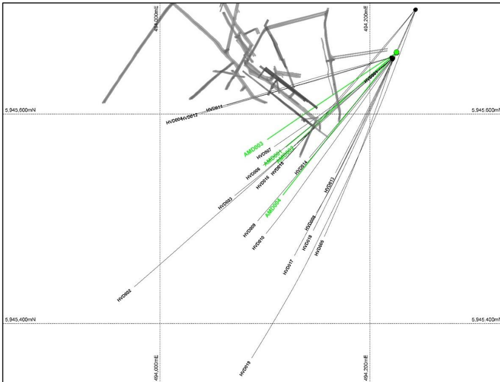
Figure 6. Plan view showing locations of recent Advance Metals holes AMD001-004 (green) in reference to previous drill holes (black) and historic workings (grey) at the Happy Valley Prospect at Myrtleford.
