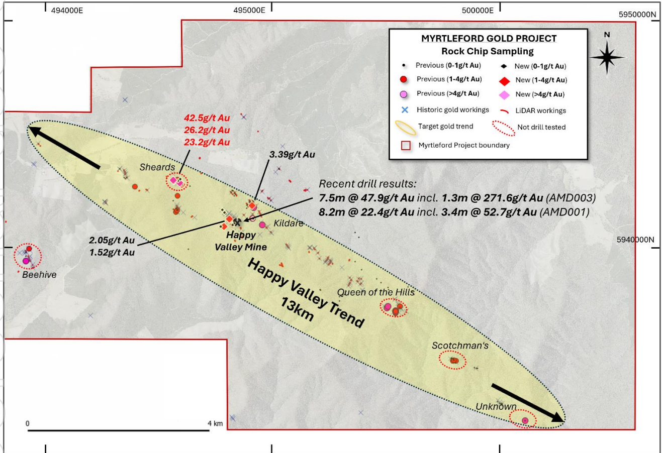
Figure 3. Plan of the southeastern portion of the Myrtleford Project highlighting previous (ASX AVM 17 January 2025) and new rock chip sampling at over the Happy Valley Trend. Full details of recent rock chip sampling is provided in Table 3 .
