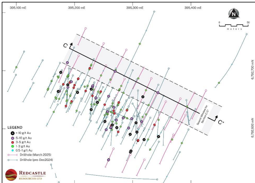
Plan view showing search window of 55m centred on section line C-C'
