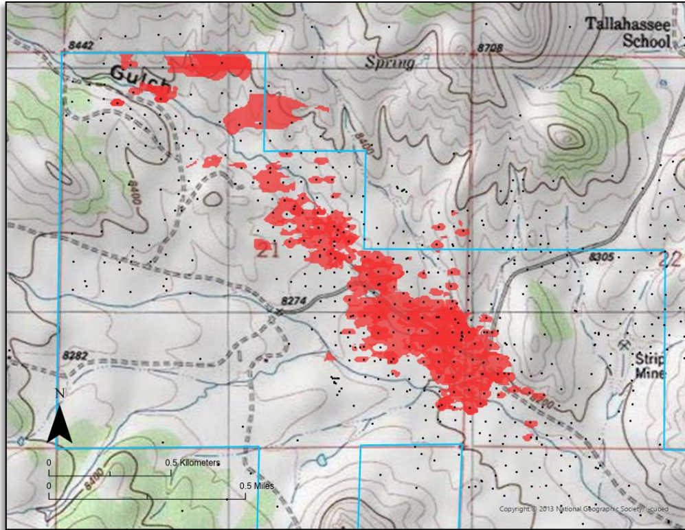
Figure 7: Plan view of the 0.075% U 3 O 8 grade shells
