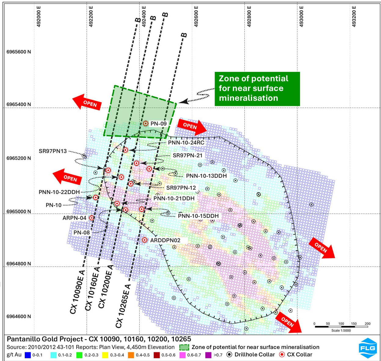
Figure 2: Pantanillo Gold Project – Drillhole Collar and Section Plan
