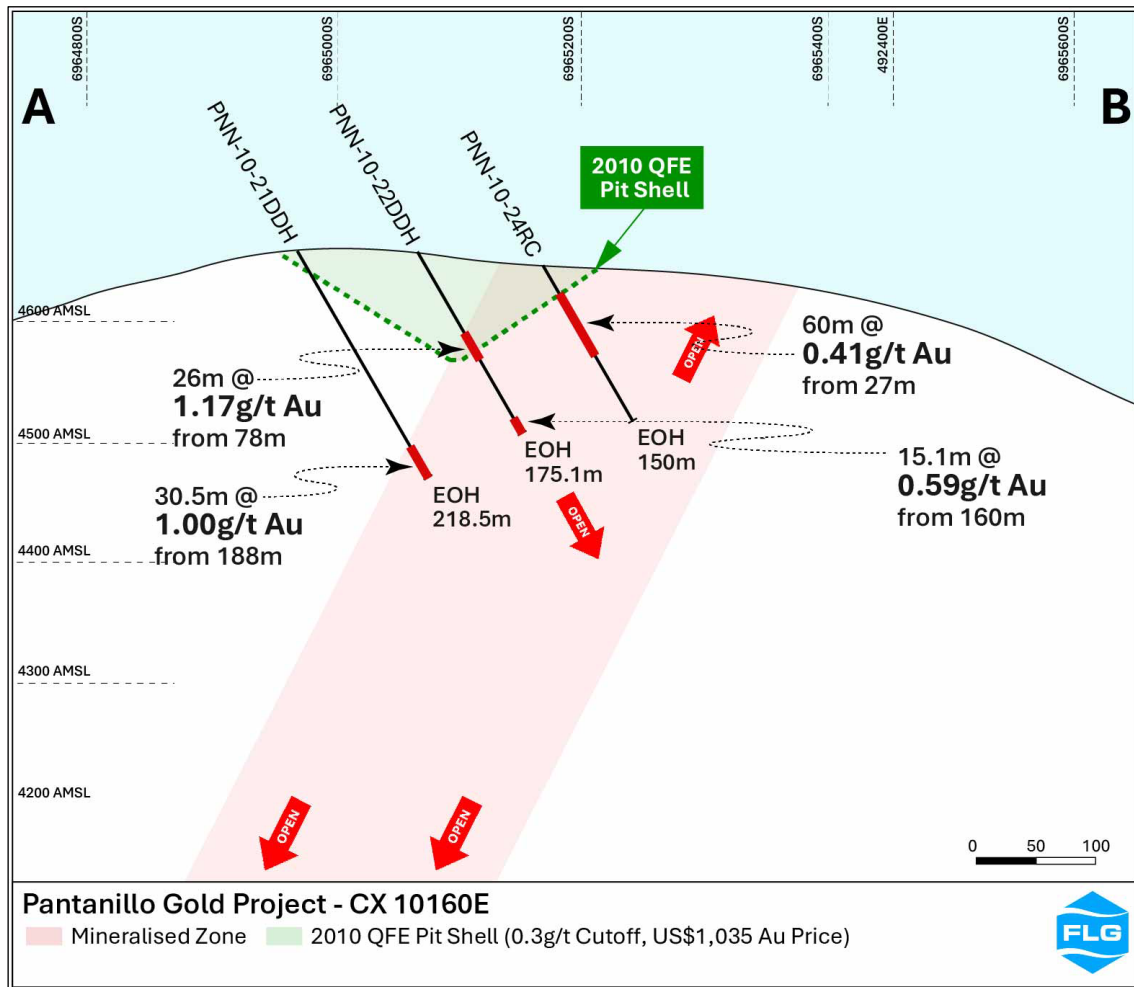
Figure 4: Pantanillo Gold Project – Cross Section 10160E
