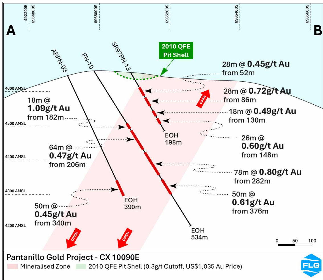
Figure 3: Pantanillo Gold Project – Cross Section 10090E
