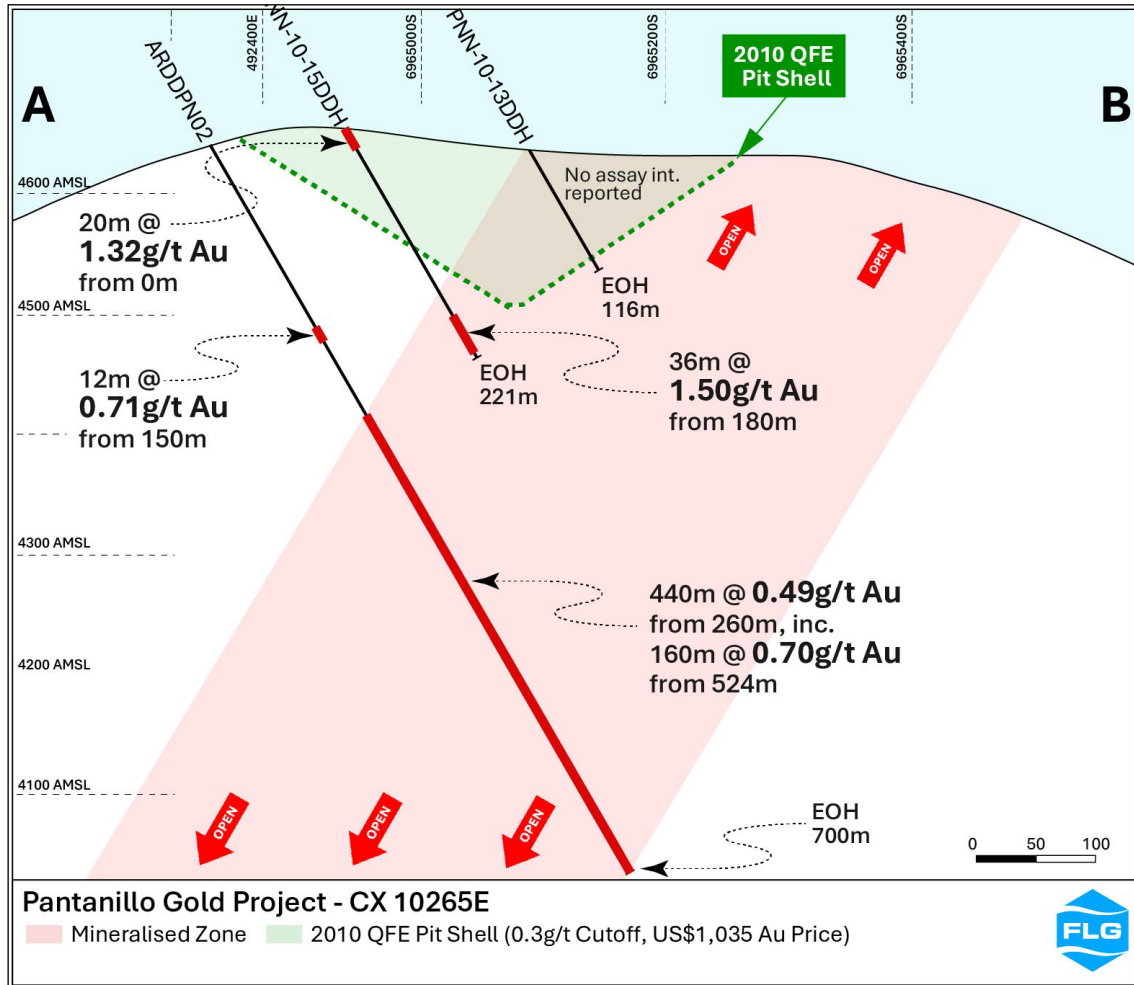
Figure 6: Pantanillo Gold Project – Cross Section 10265E
