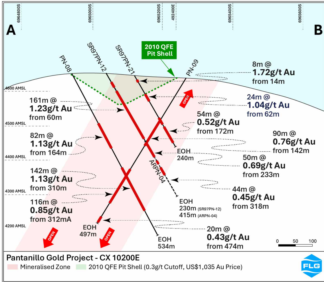
Figure 5: Pantanillo Gold Project – Cross Section 10200E
