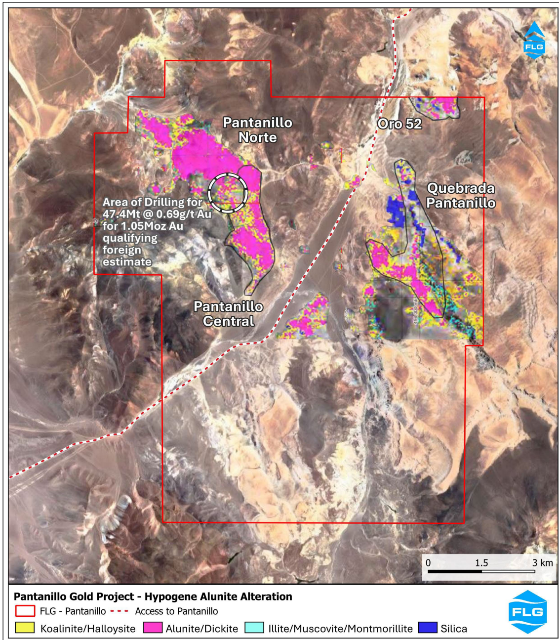
Figure 7: Pantanillo Gold Project – Aster Imaging & Exploration Potential
