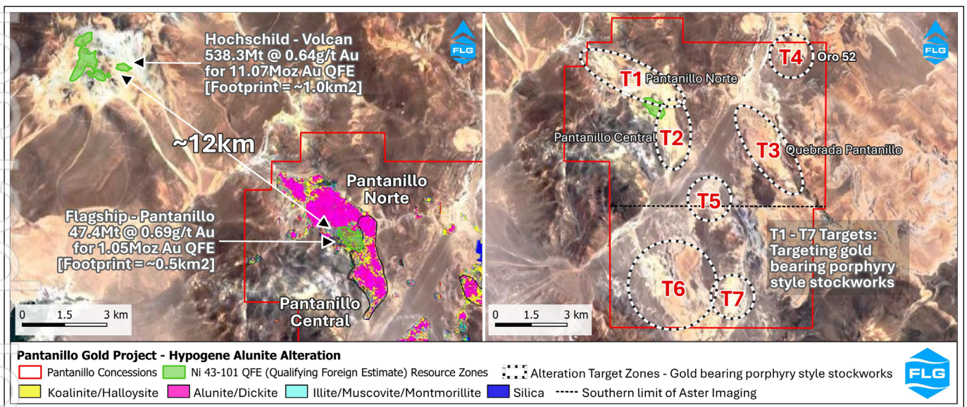
Figure 7: Pantanillo Gold Project – Exploration Potential
