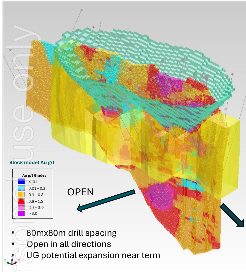
3D model with AUD $5000 Pit shells, block model and mineralised wireframes
