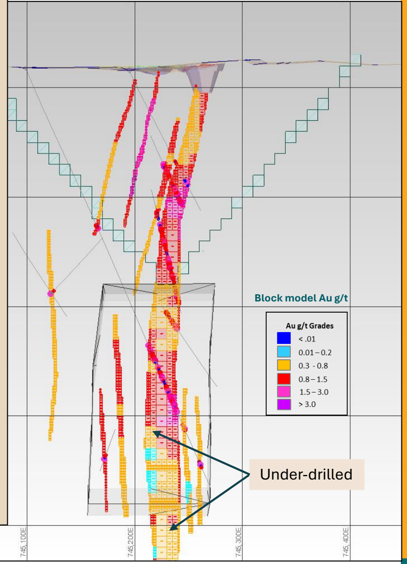
Cross section of Block model with AUD $5000 pit shell slice
