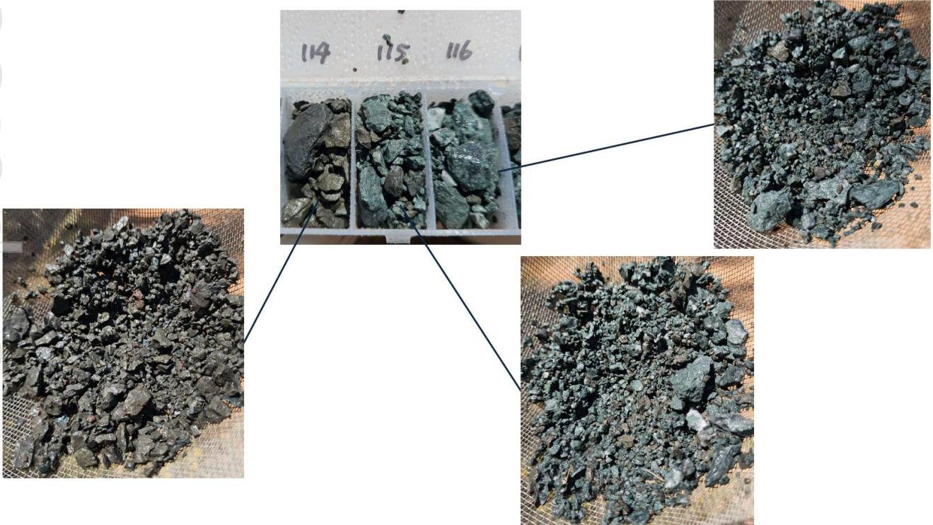
Figure 8: Massive sulphide pyrite-chalcopyrite-sphalerite in RC drill chips at 114 to 116m in hole GCC0004
