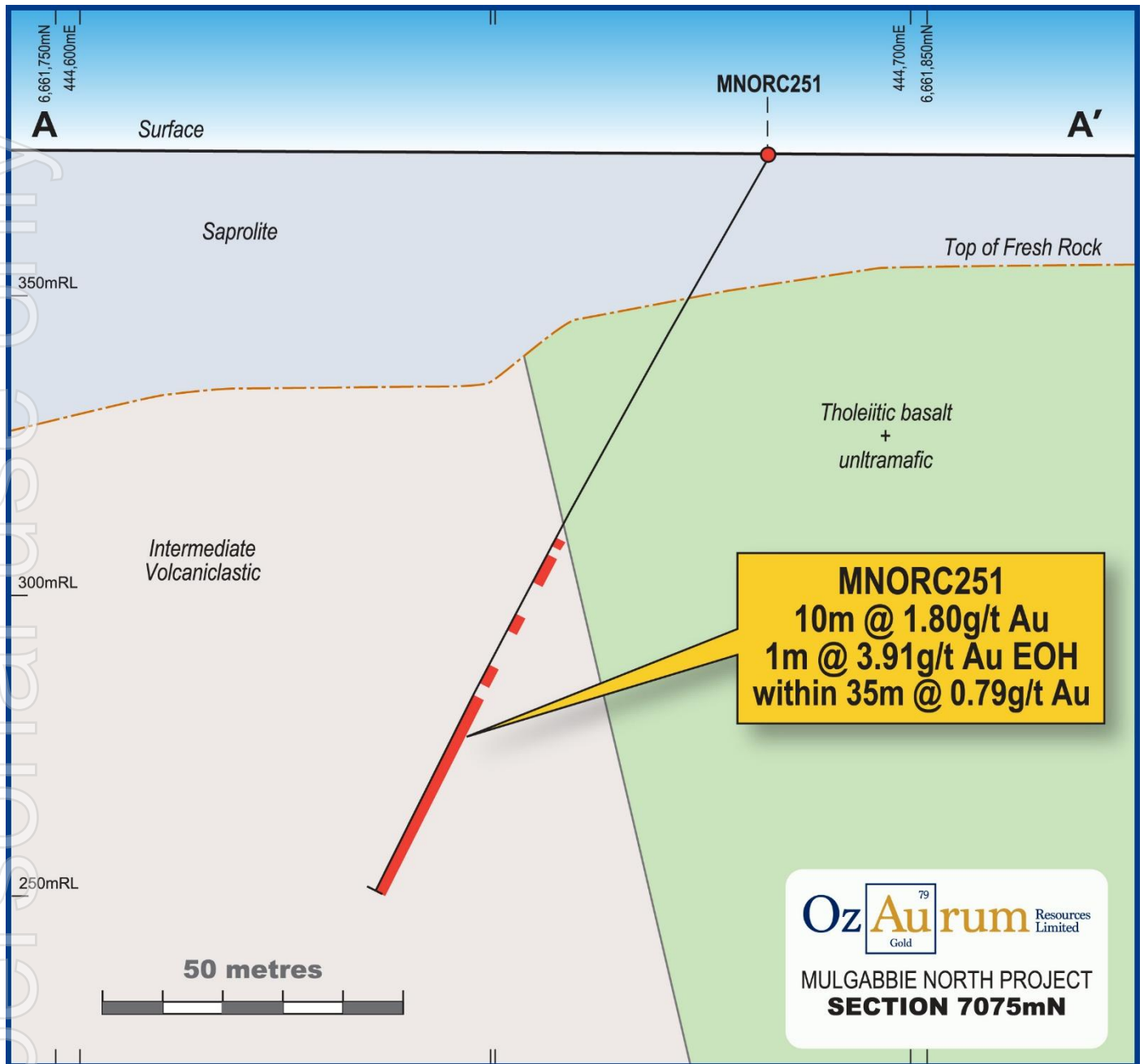
Figure 2: Cross Fault cross section 7075N
