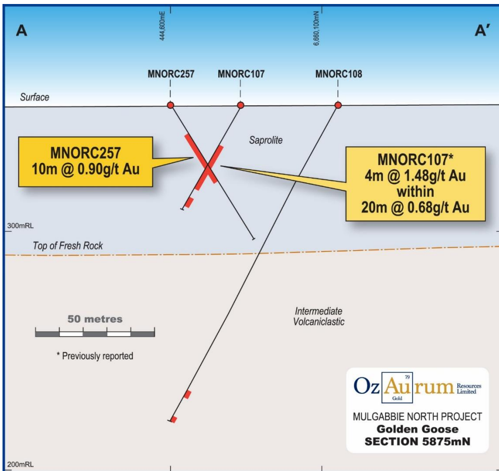
Figure 4: Golden Goose cross section 5875N
