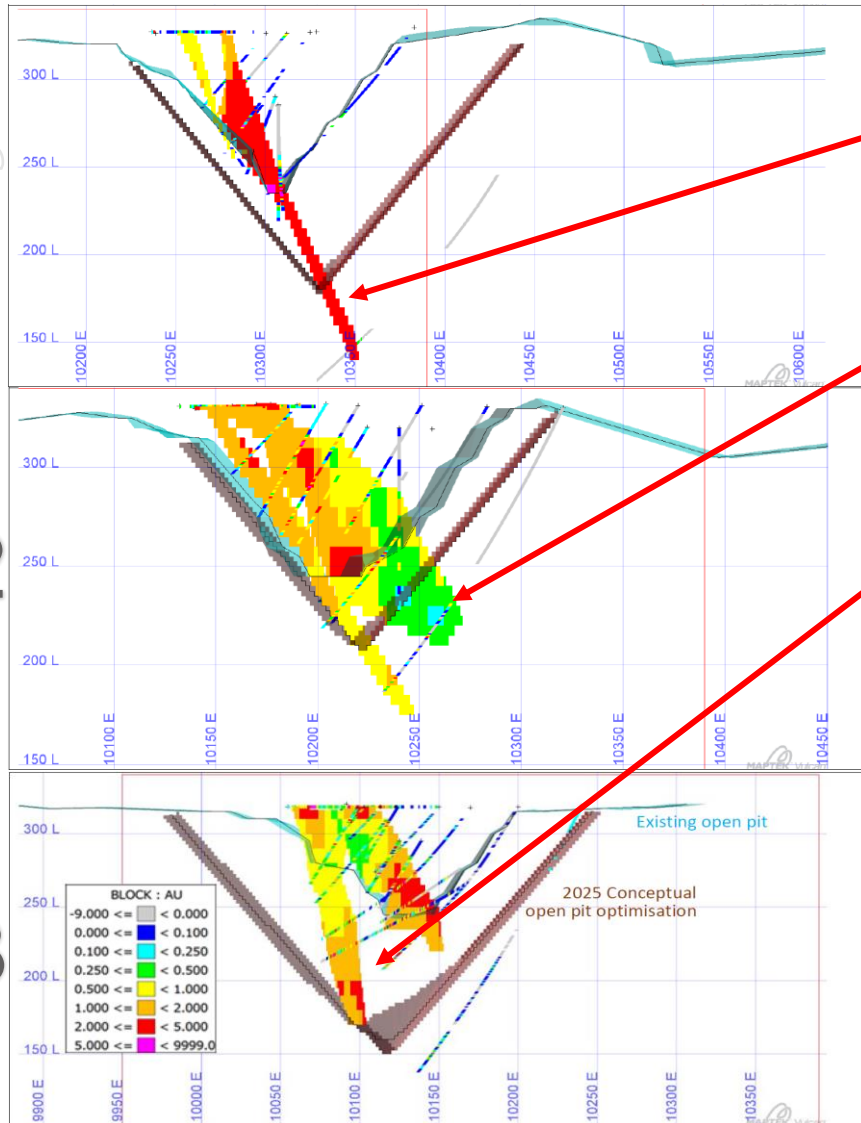
West-east section w/ drill holes, resource model, existing pit and conceptual pit for reporting.
