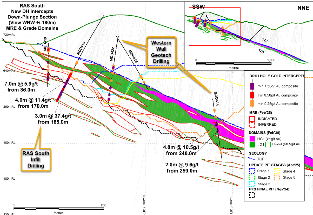
Figure 3. RAS South Down-Plunge Section
