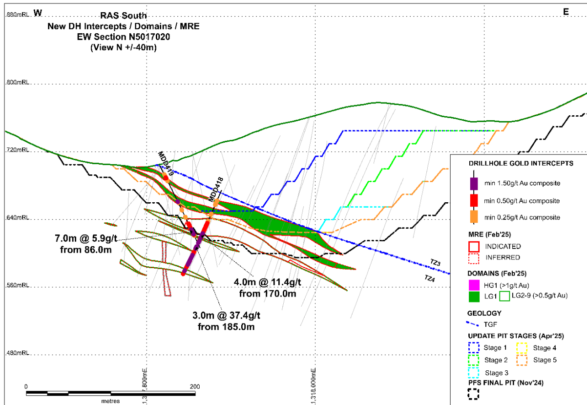
Figure 2. RAS South EW X-Section N5017020
