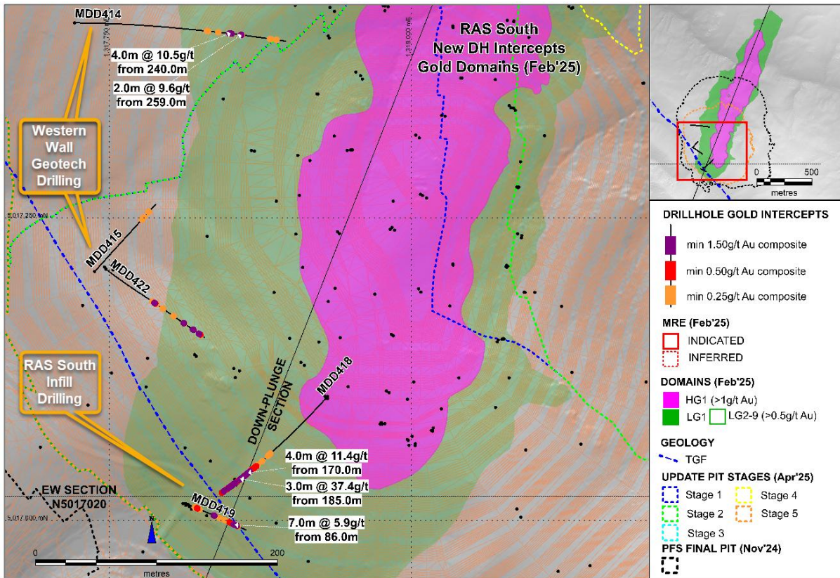
Figure 1. Plan of RAS South new drilling intercepts
