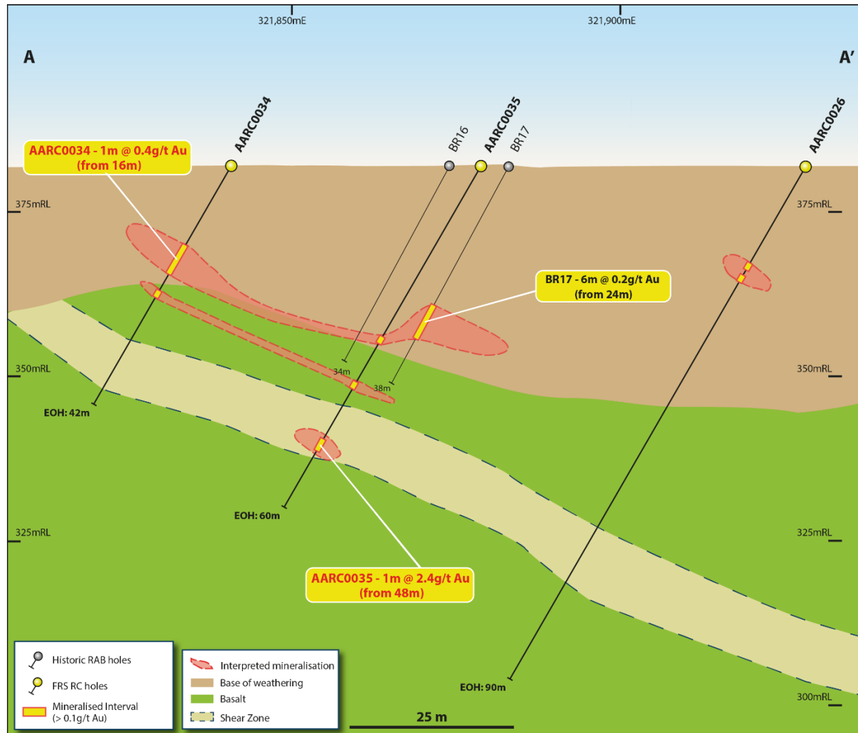
Figure 9. Cross section (A-A'), looking north, ~10m section view, showing interpreted geology and Au mineralisation of historic drilling. Drilling results are down hole width and not true width.
