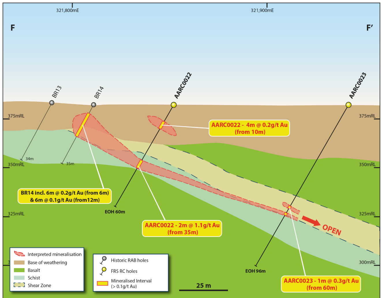
Figure 7. Cross section (F-F'), looking north, ~5m section view, showing interpreted geology and Au mineralisation of historic drilling. Drilling results are down hole width and not true width.
