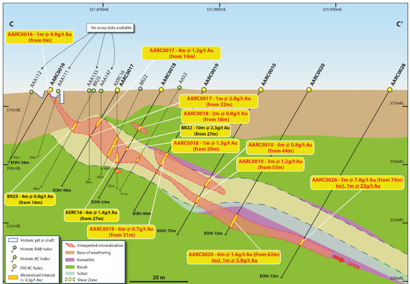
Figure 4. Cross section (C-C'), looking north, ~10m section view, showing interpreted geology and Au mineralisation of historic drilling (black text) and significant, recent FRS drilling (red text). Drilling results are down hole width and not true width.
