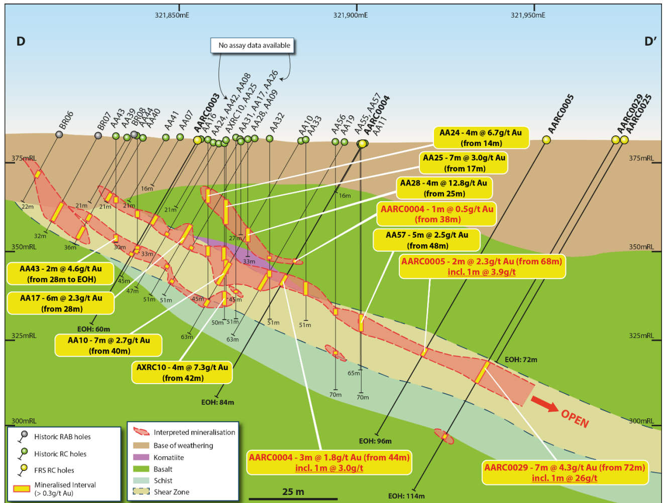
Figure 5. Cross section (D-D'), looking north, ~10m section view, showing interpreted geology and Au mineralisation of historic drilling (black text) and significant, recent FRS drilling (red text). Drilling results are down hole width and not true width.
