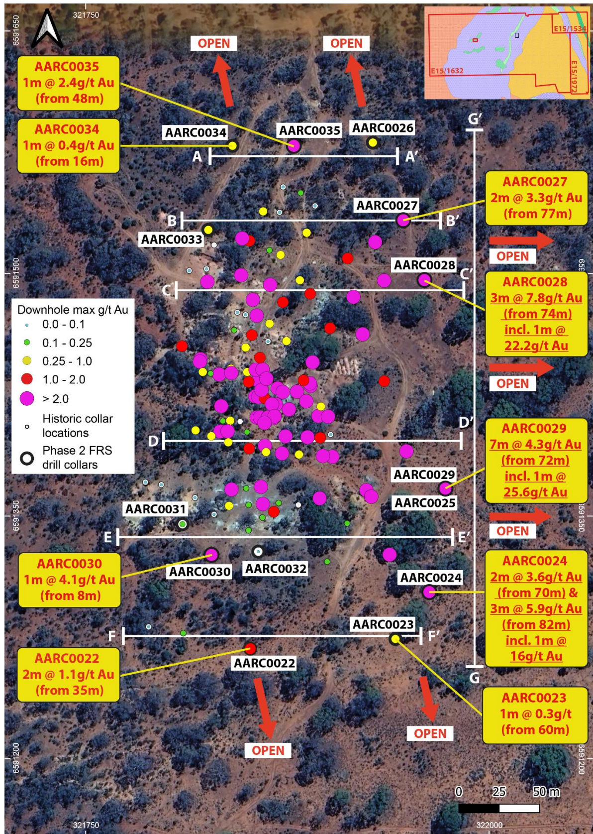
Figure 2. Historic and recent downhole max results at the Ada Ann prospect with significant FRS phase 2 results indicated, along with location of cross and long sections (which can be seen below and within the supplementary data). Drilling results are down hole width and not true width.
