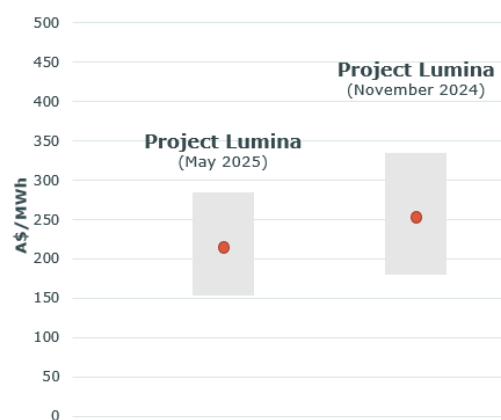
Figure 1 – Project Lumina LCOS range (8-hour storage duration)
