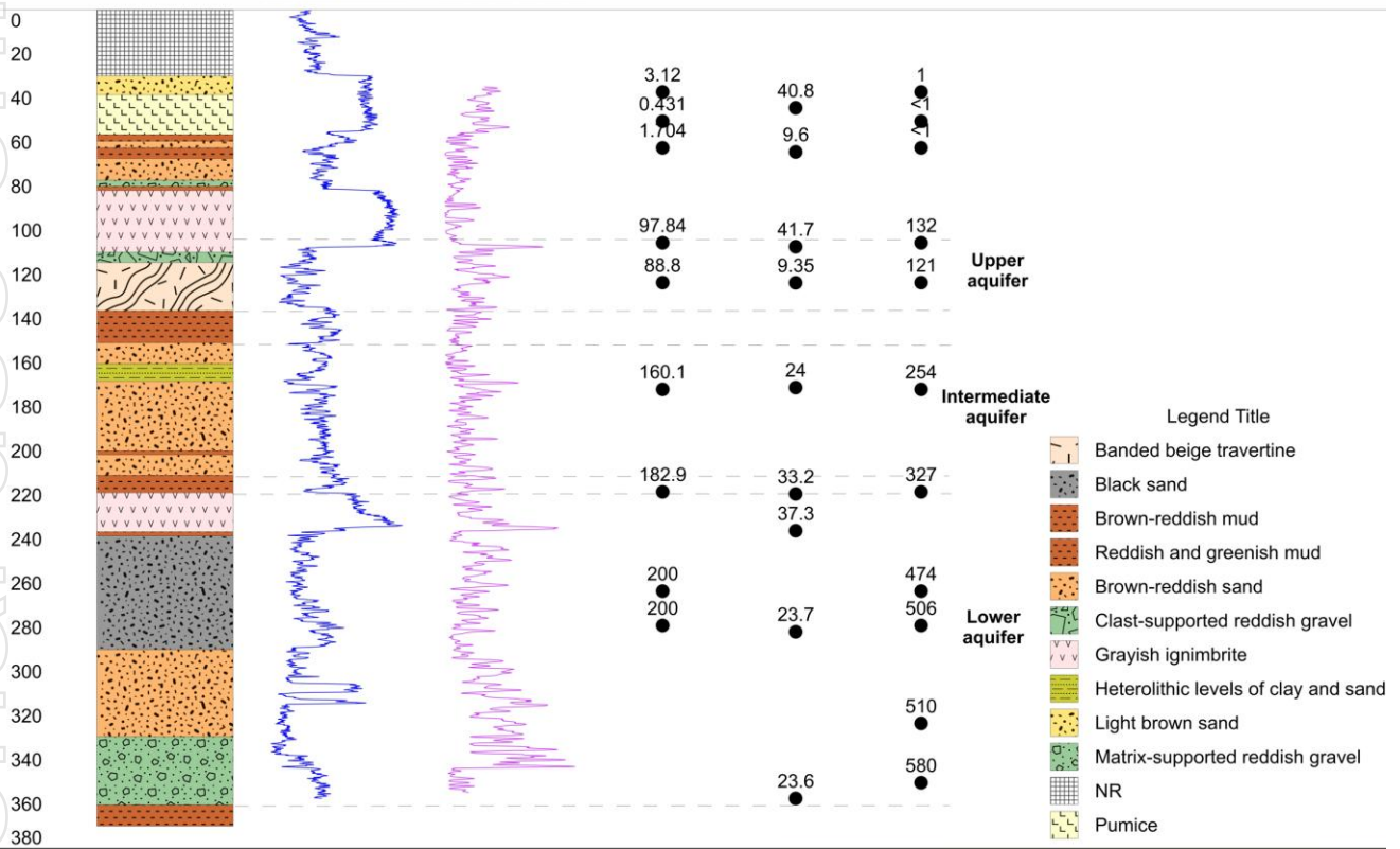
Figure 1. Vertical scale in metres. Three aquifer zones delineated by specific yield- the average value of total porosity (TPOR) and specific yield (SY) is 28% and 9% respectively throughout the entire recorded interval.
