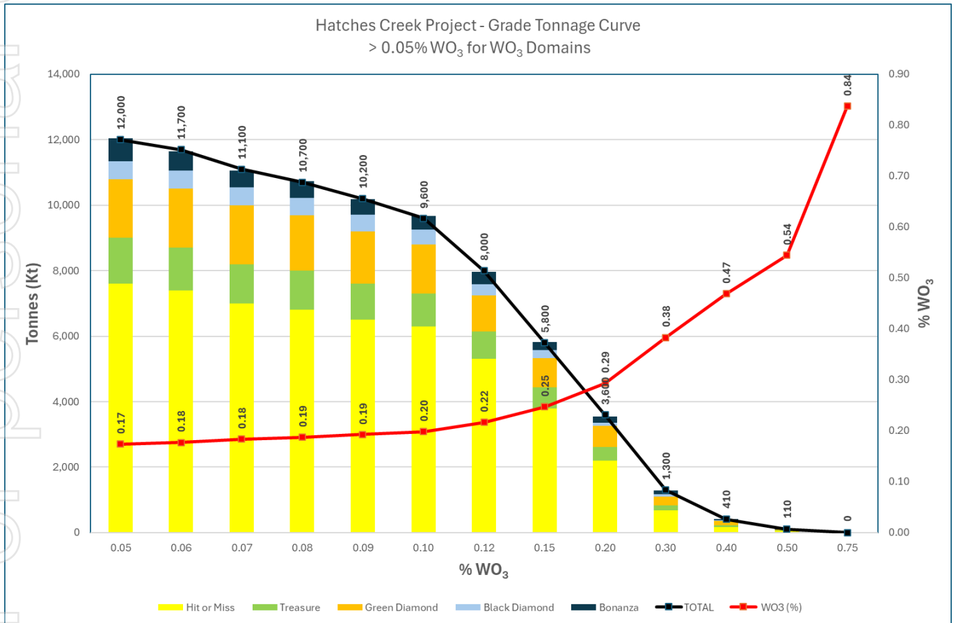
Figure 12. Grade tonnage curve for the Hatches Creek WO 3 domains.
