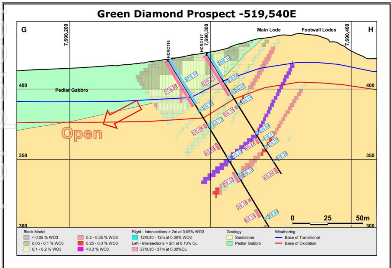
Figure 9. Section G-H showing multiple zones of tungsten and copper mineralisation at Green Diamond. Note substantial widths in HCRC116 open at depth.
