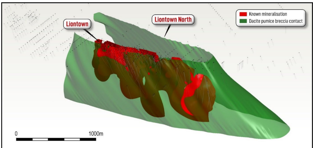
Figure 3: 3D model of the eastern end of the Liontown Dome, showing the prospective contact (green) and the Resource at Liontown (red).
