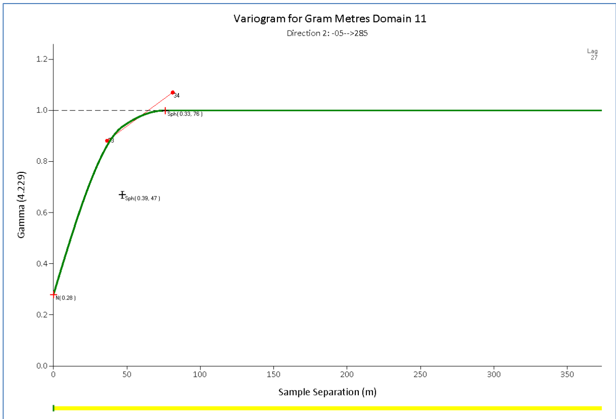
Figure 23: Majestic North Project, Domain 11, Gram-Metres Variogram, Direction 2.
