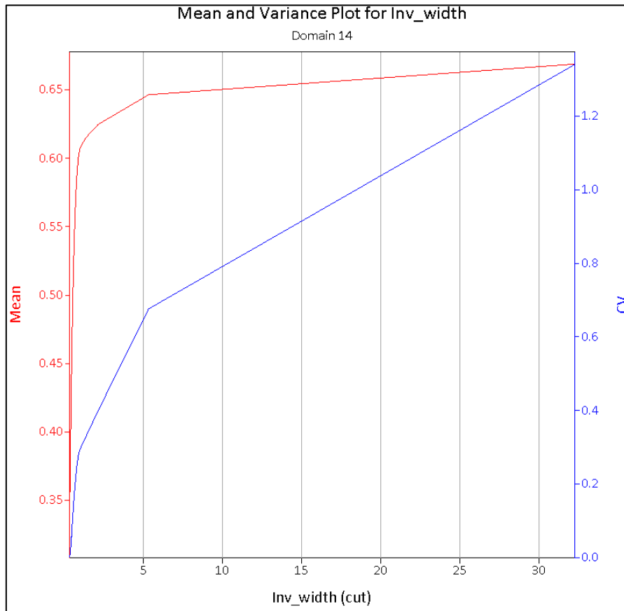
Figure 16: Mean and Variance Plot for Inverse-Width, Domain 14.
