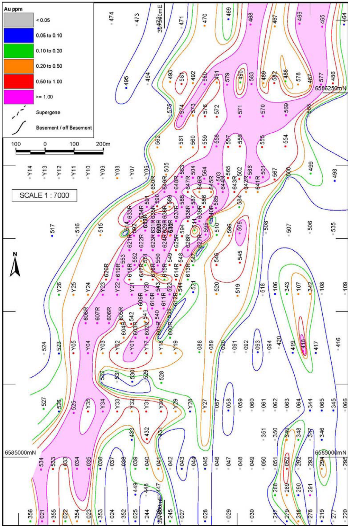
Figure 3: Combined best gold result for the Majestic North AC and RC drilling. (Early Gindalbie drilling has grade arithmetically concentrated from 4m composite to 1m).
