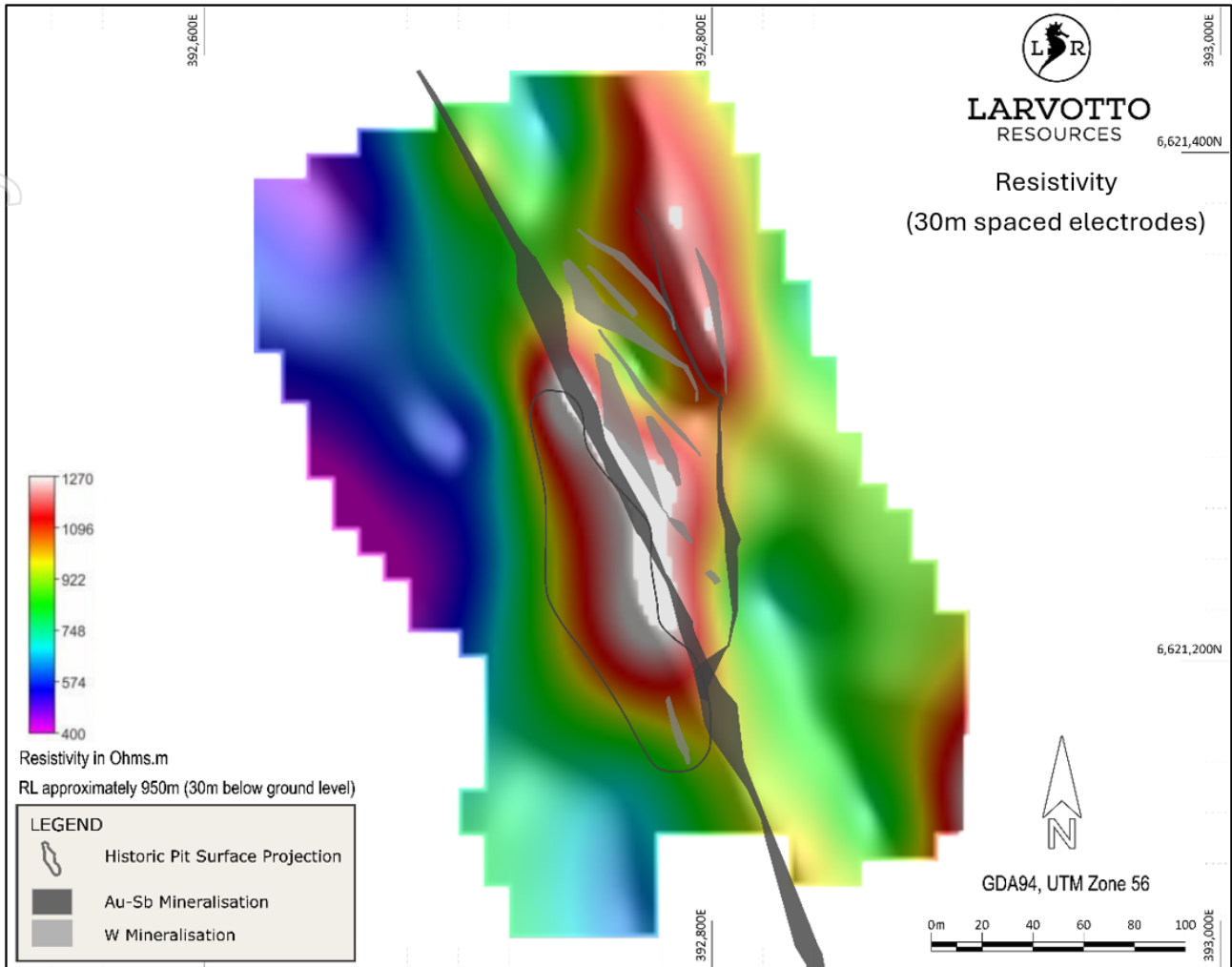
Figure 2 Colourised contours for resistivity (30m spaced electrodes) measurements at -30m from topographic surface. Modelled mineralisation is shown at the same level (-30m from topographic surface).
