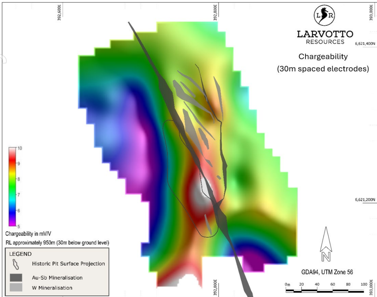
Figure 3 Colourised contours for chargeability (30m spaced electrodes) measurements at -30m from topographic surface. Modelled mineralisation is shown at the same level (-30m from topographic surface).
