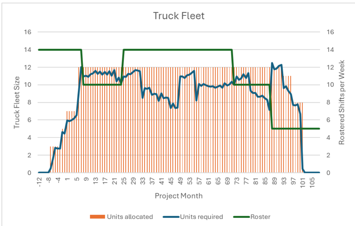
Figure 16: Truck Fleet
