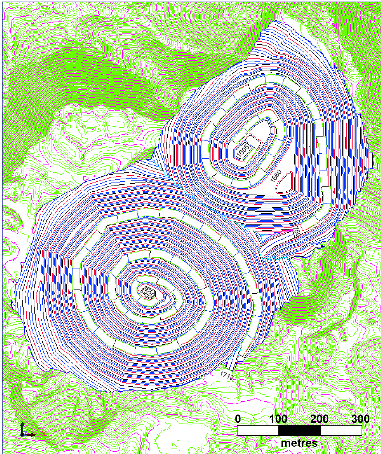
Figure 13: Stage 3 Pit
