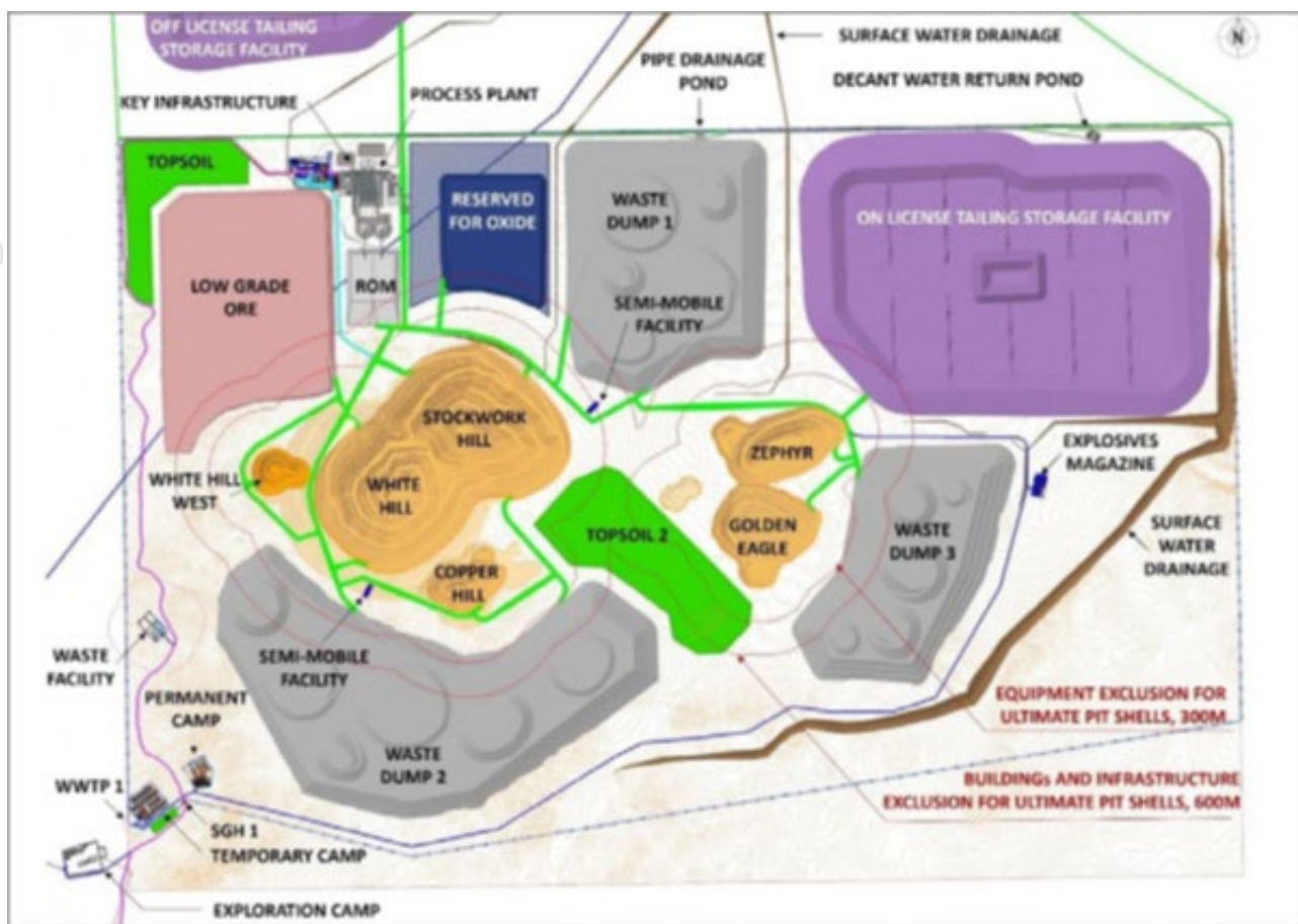
Figure 4-4: Kharmagtai proposed site layout.
