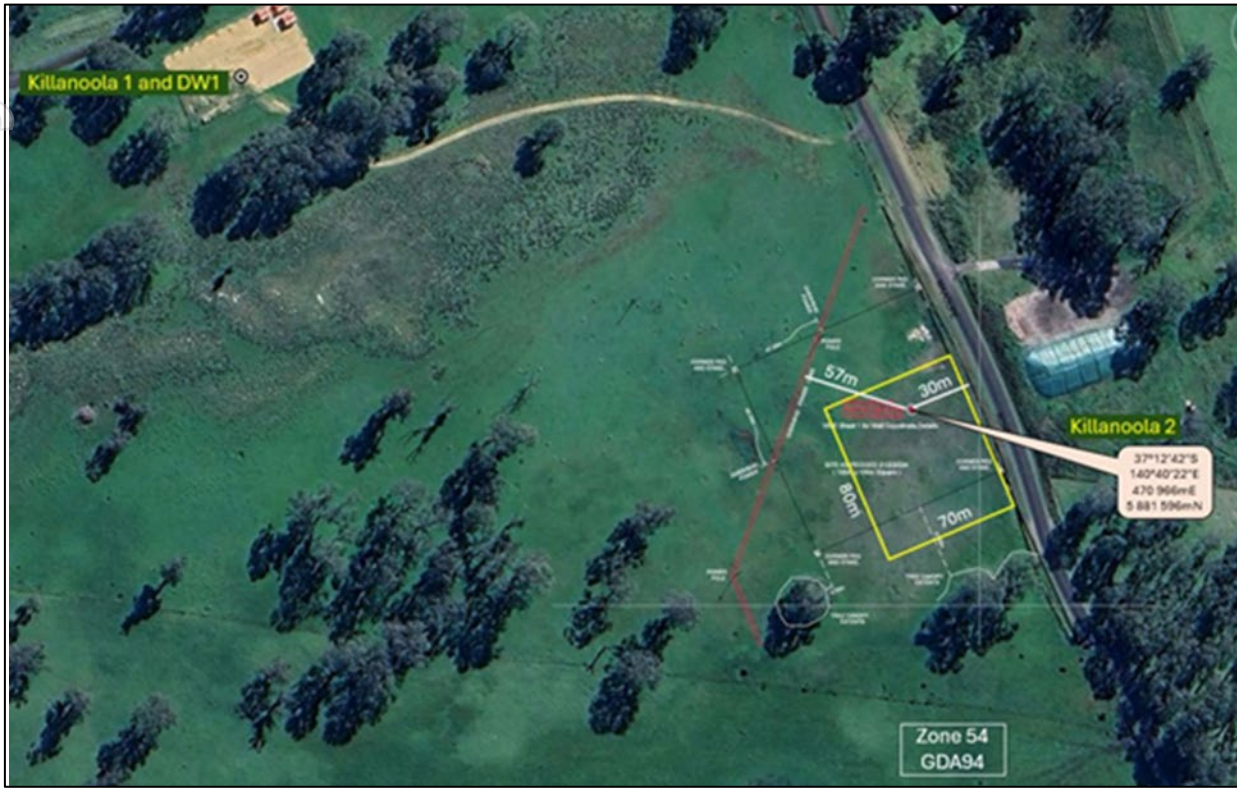
Figure 2: Location of well pad to be built at KN2
