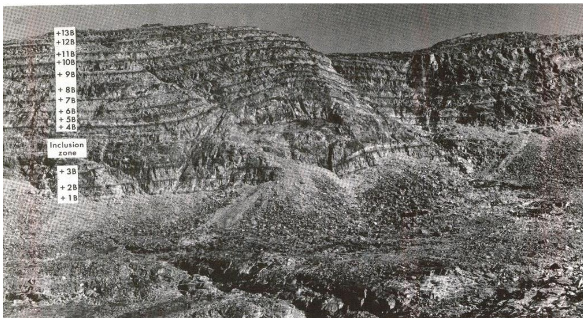
Figures 2 Showing the Kakortokite layered host mapped a stratigraphic column over a 400m vertical face. The Fjord MRE lies at the base of the measured column and extends over 50m below ground. The Kakortokite stratigraphic column was mapped and has not been sampled. The Kakortokite host does not indicate any certainty of hosting economic mineralization.
