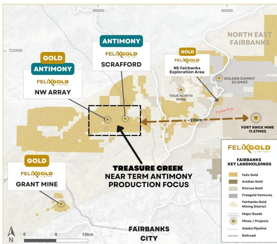
Fig 1. Location of Treasure Creek with near-term antimony production focus
