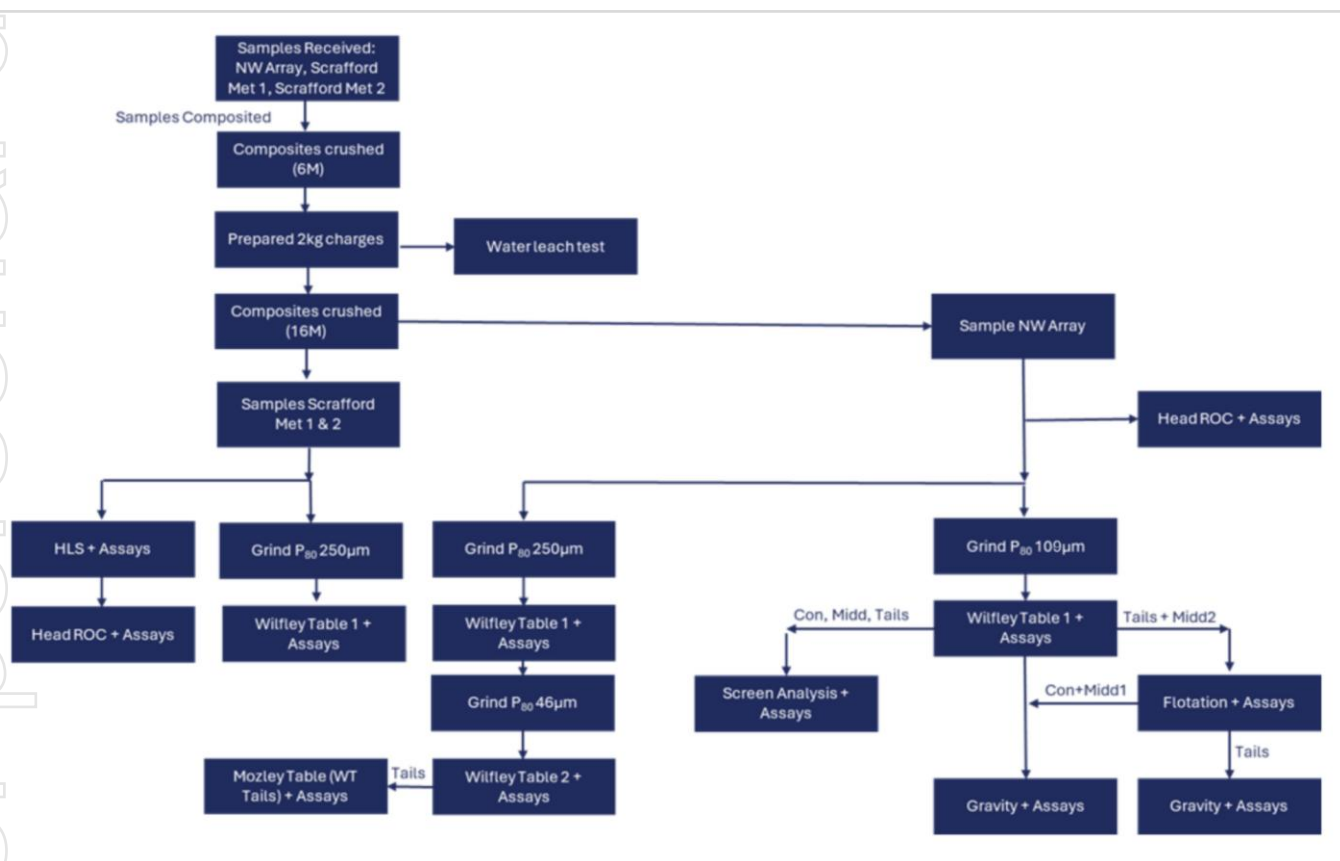
Fig 2. Workflow for Metallurgical Test Work Program
