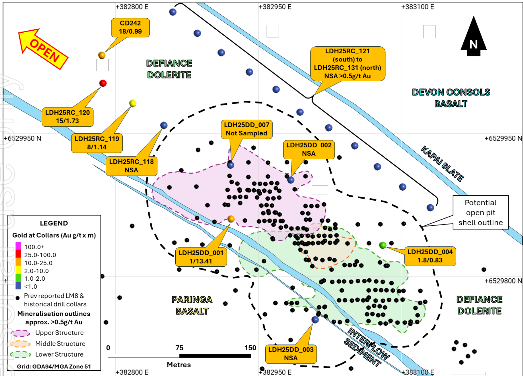
Figure 1: Plan View of the Lady Herial potential development footprint illustrating recent Company (LDH) drill holes (previous holes have all been reported – see page 7 for dates of relevant Lady Herial announcements).
