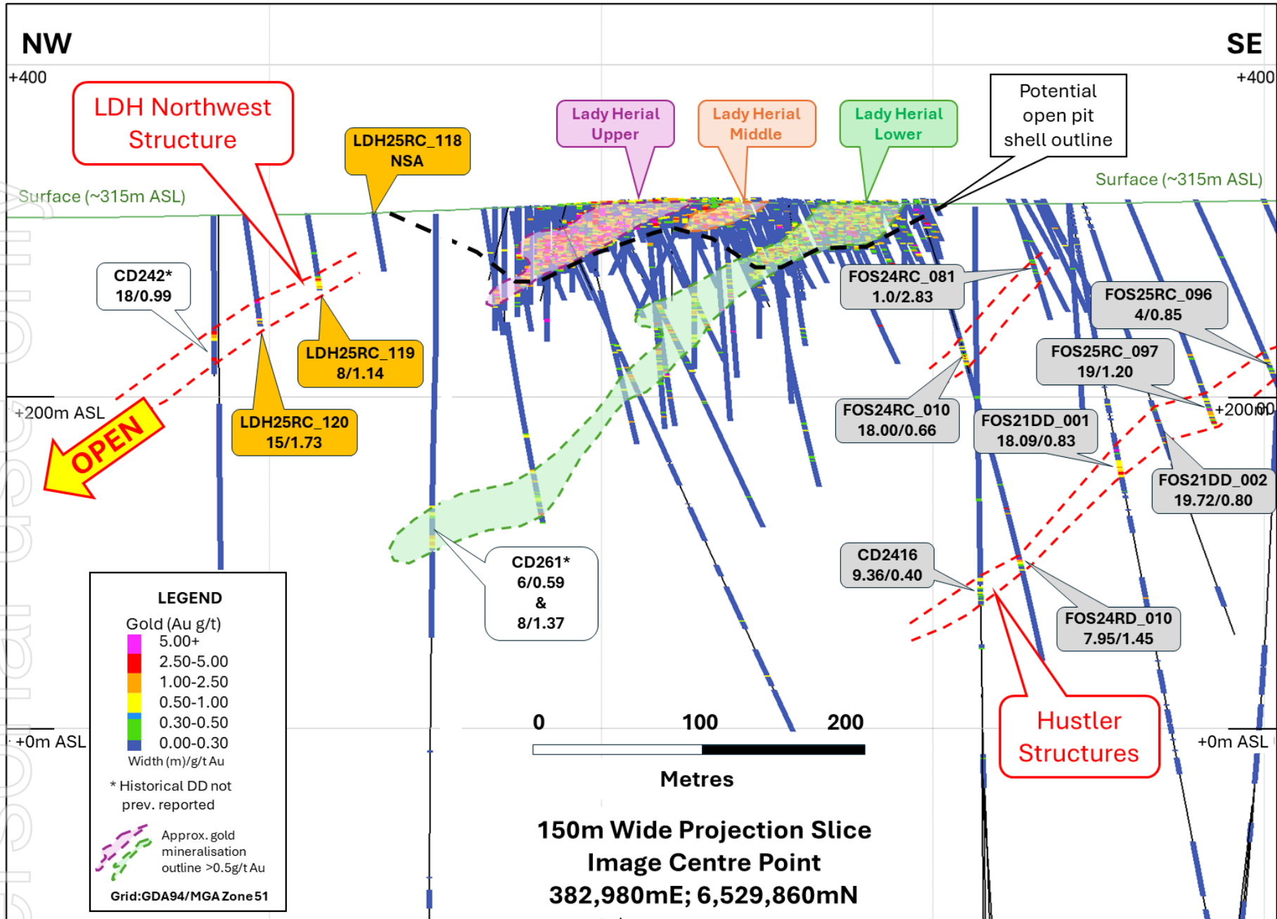
Figure 2: Cross sectional projection view of the Lady Herial deposit illustrating recent sterilisation drill holes (orange call-outs) and select local holes on other structures previously reported (grey callouts – ASX announcements dated 10 Oct & 13 Dec 2024 and 18 Mar 2025).
