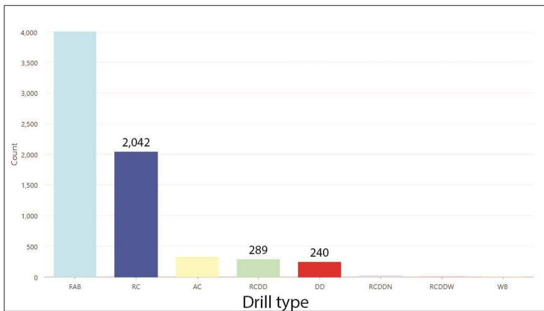
Figure 3.8: Histogram of drillhole by type
