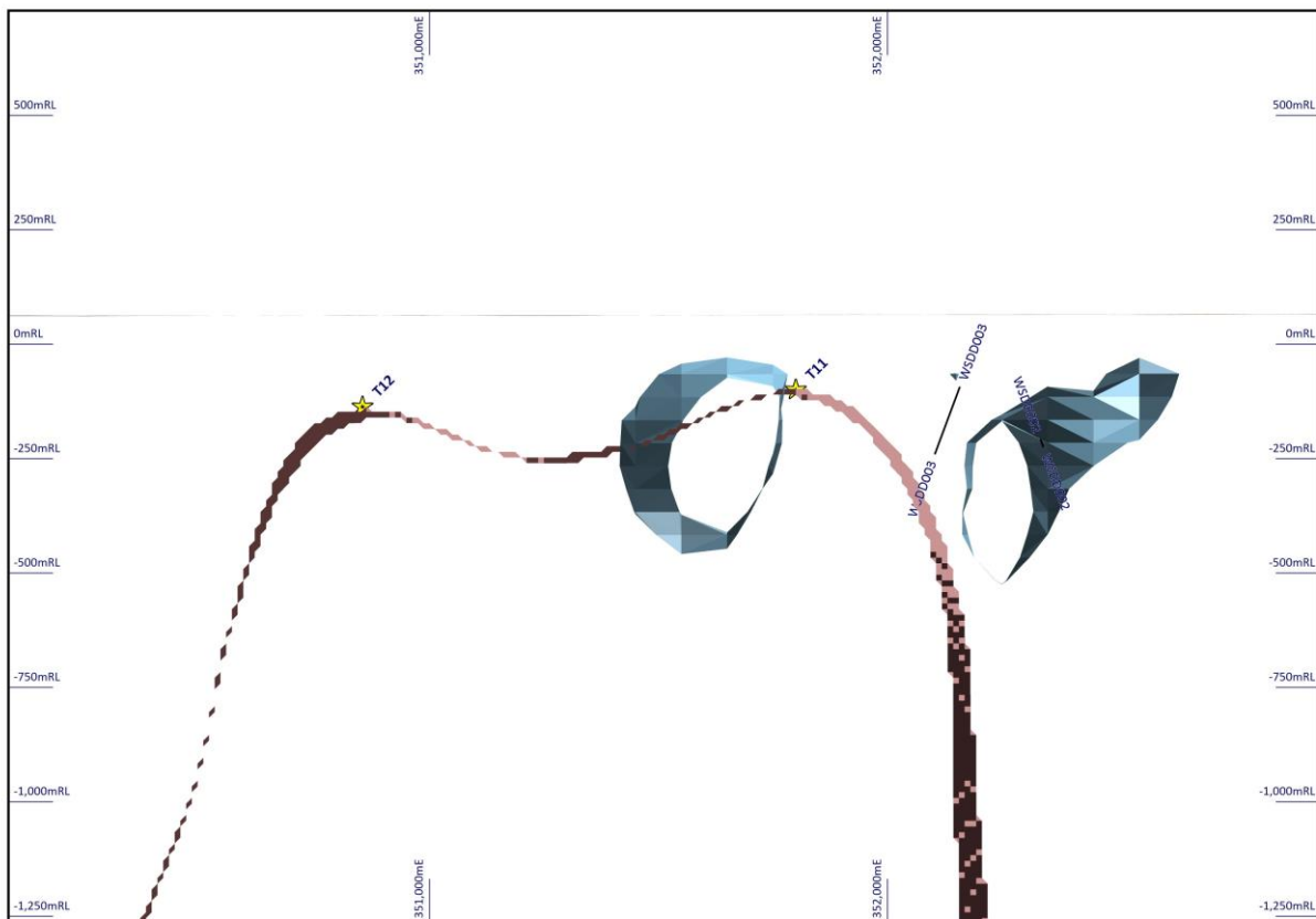
Figure 3. Cross Section of T11 and T12 Targets (looking north) showing overlapping magnetic (pink) and gravity (blue) inversion models in proximity to 2023 diamond hole WSD003.
