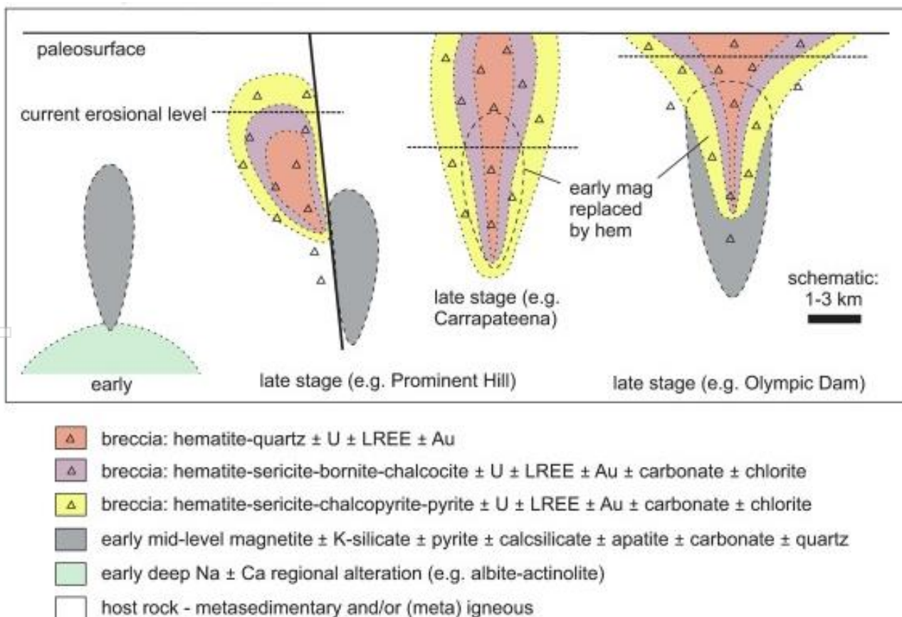
Figure 4. Examples of IOCG deposits showing relationship between early and/or deeper magnetite and later and/or shallower hematite mineralisation (Skirrow, 2022).
