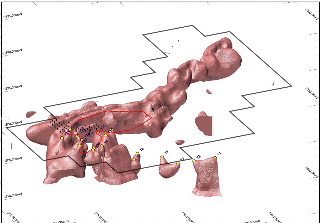
Figure 1. Oblique view (looking southwest) of Whaleshark magnetic inversion model and new targets in relation to granodiorite pluton (red polygon) and drilling (black dots).
