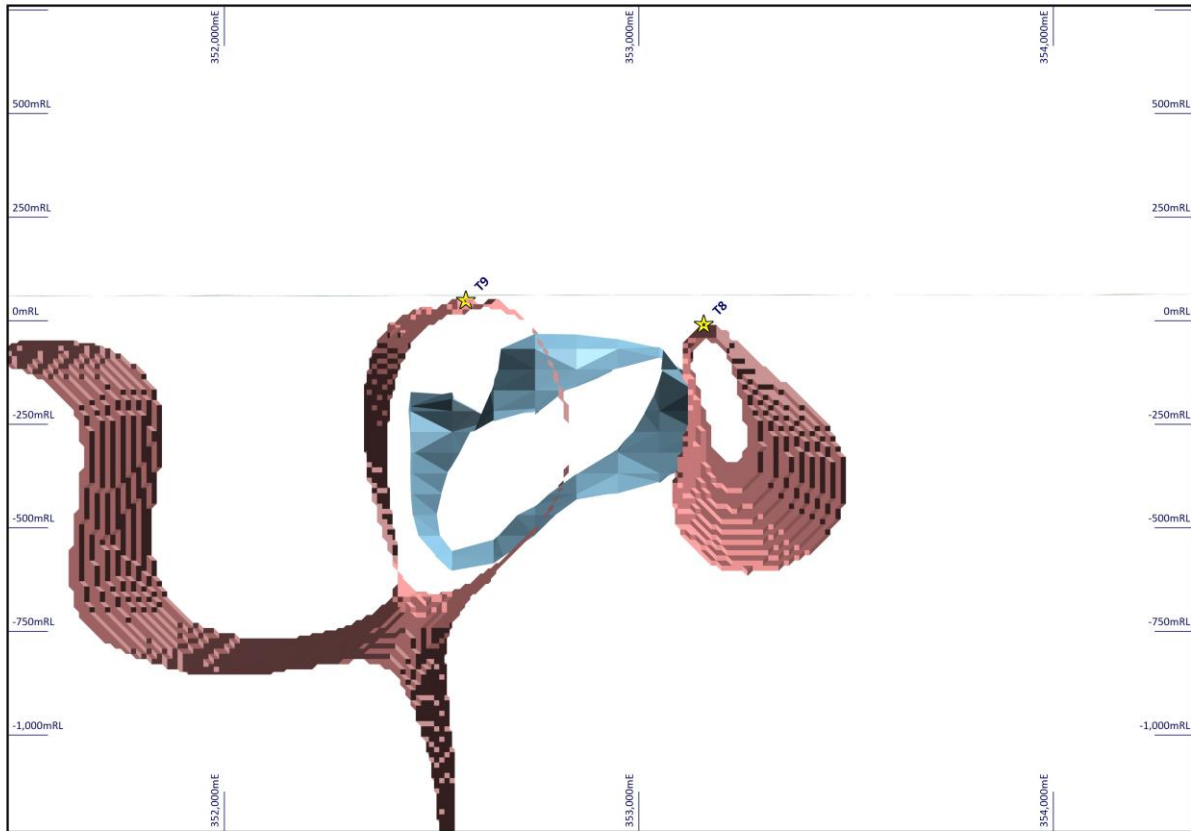
Figure 2. Cross Section of T8 and T9 Targets (looking north) showing overlapping magnetic (pink) and gravity (blue) inversion models.
