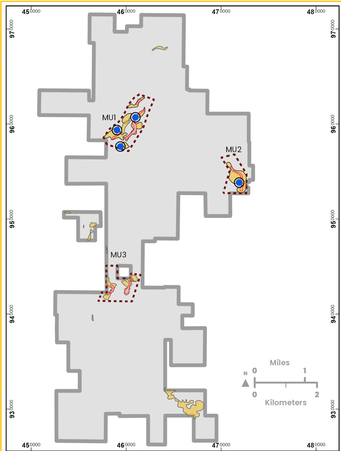
FIGURE 10: RESOURCE AREAS, MONITOR WELLS, AND PROPOSED MINE UNITS
