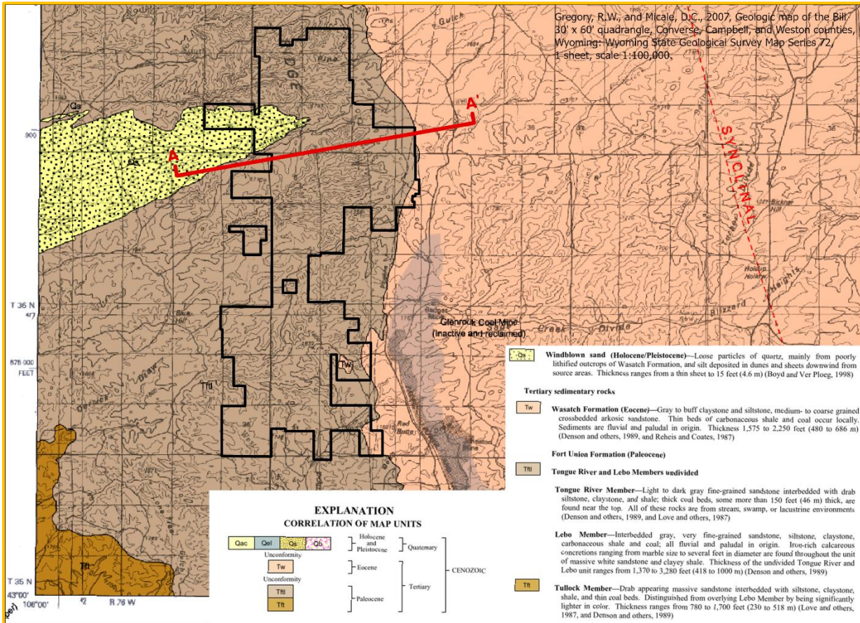
FIGURE 4: GEOLOGIC MAP, ADAPTED FROM WSGS BILL QUADRANGLE MAP (GREGORY 2007)
