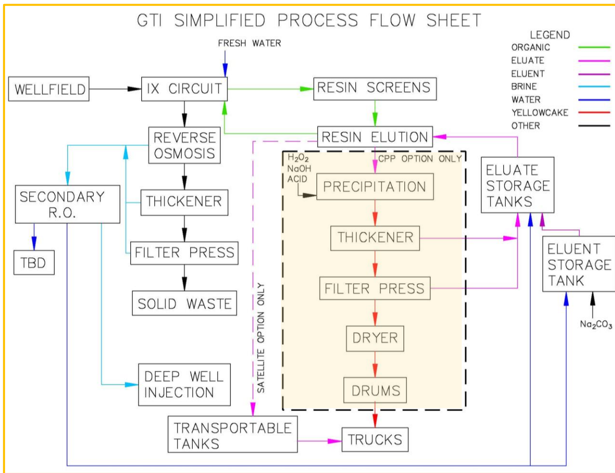
FIGURE 13: LO HERMA CPP SIMPLIFIED PROCESS FLOW SHEET
