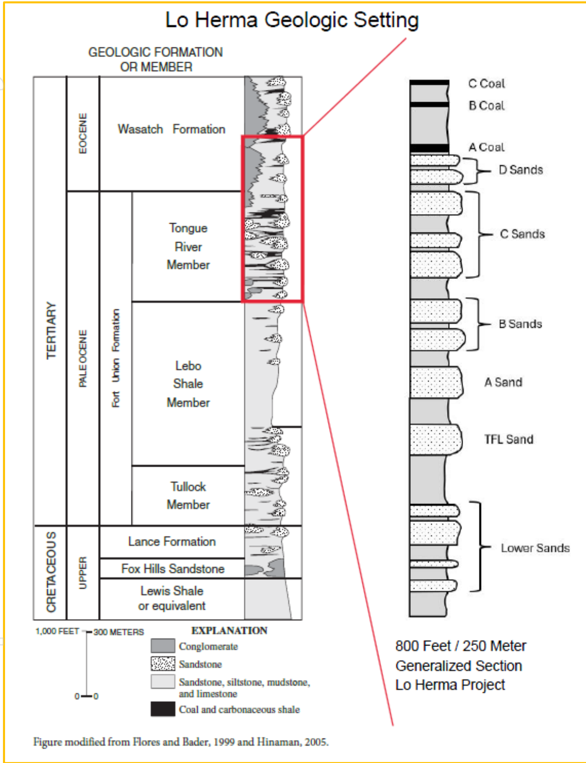
FIGURE 6: STRATIGRAPHIC SECTION
