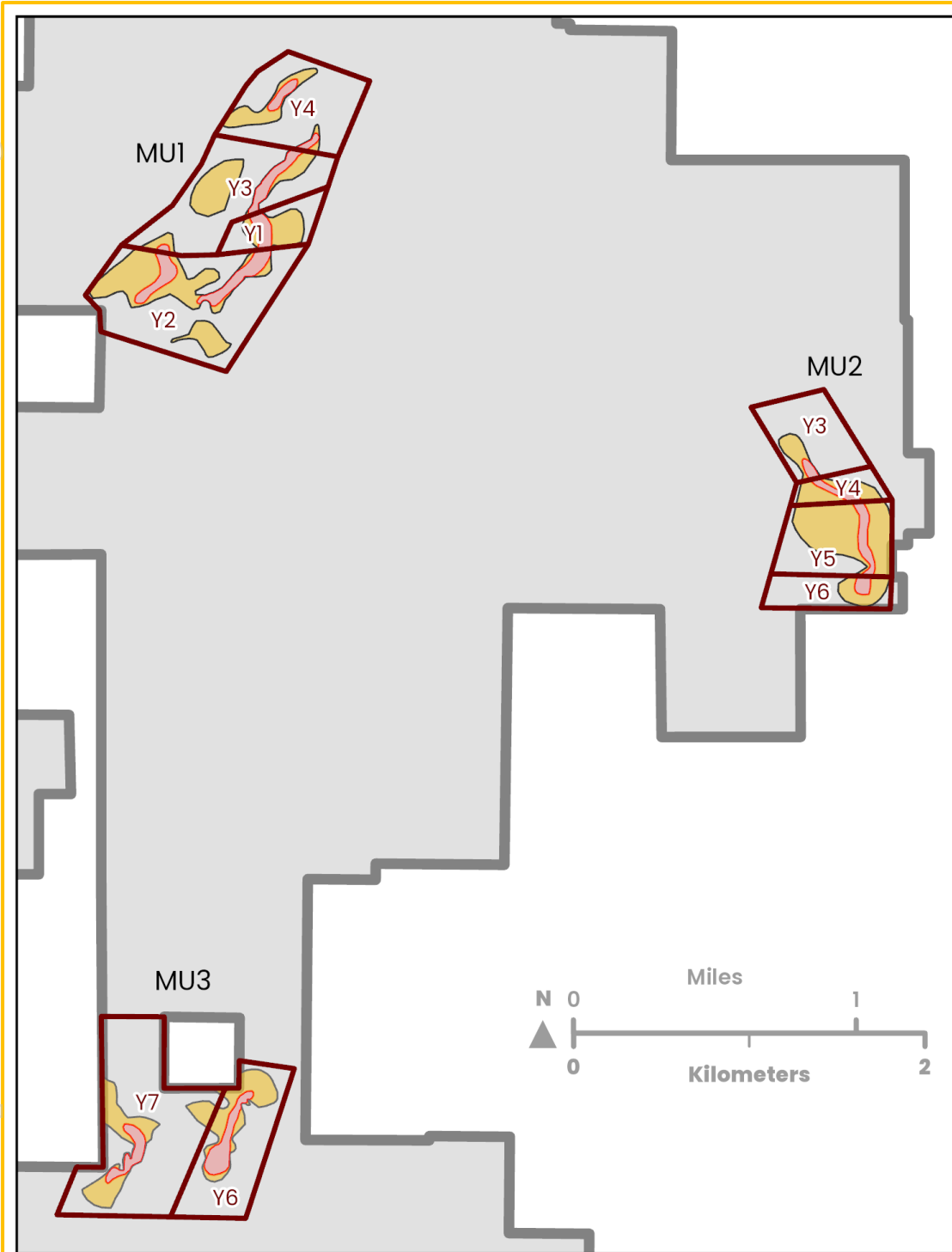
FIGURE 12: WELLFIELD DEVELOPMENT SCHEDULE, PRODUCTION YEAR NOTED ON FIGURE
