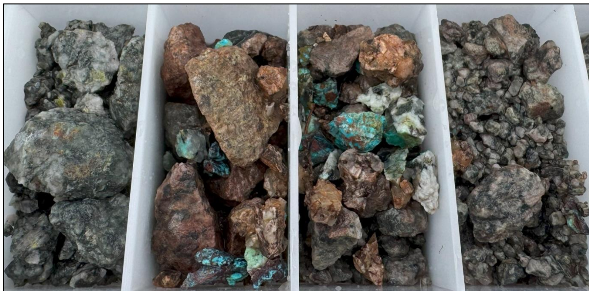
Figure 3: Copper carbonate mineralisation within an oxidised structure in PRC006 (120ft to 128 ft)
