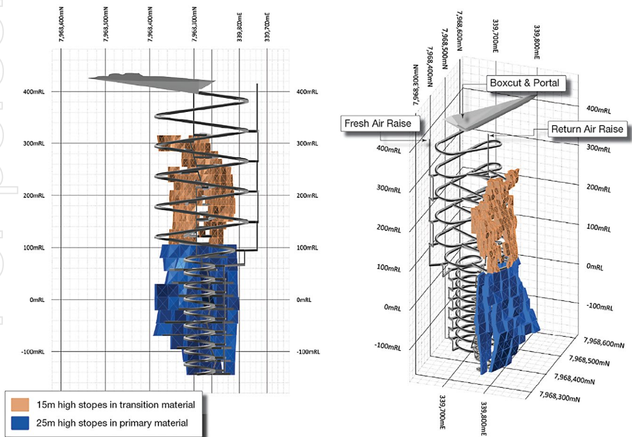
Figure 7 – Sandiego underground mine design
