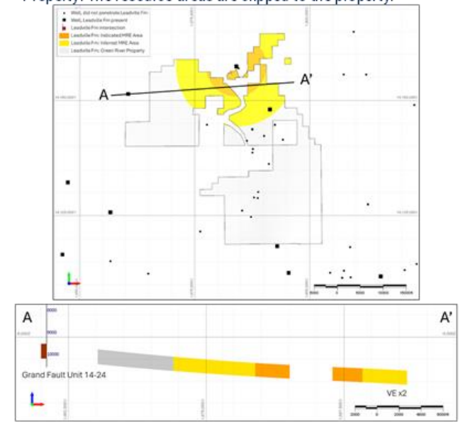
Figure 2 Cross section of the Leadville Limestone through the Inferred and Indicated MRE areas, demonstrating lateral stratigraphic and thickness continuity across the Green River Property. The resource areas are clipped to the property.
