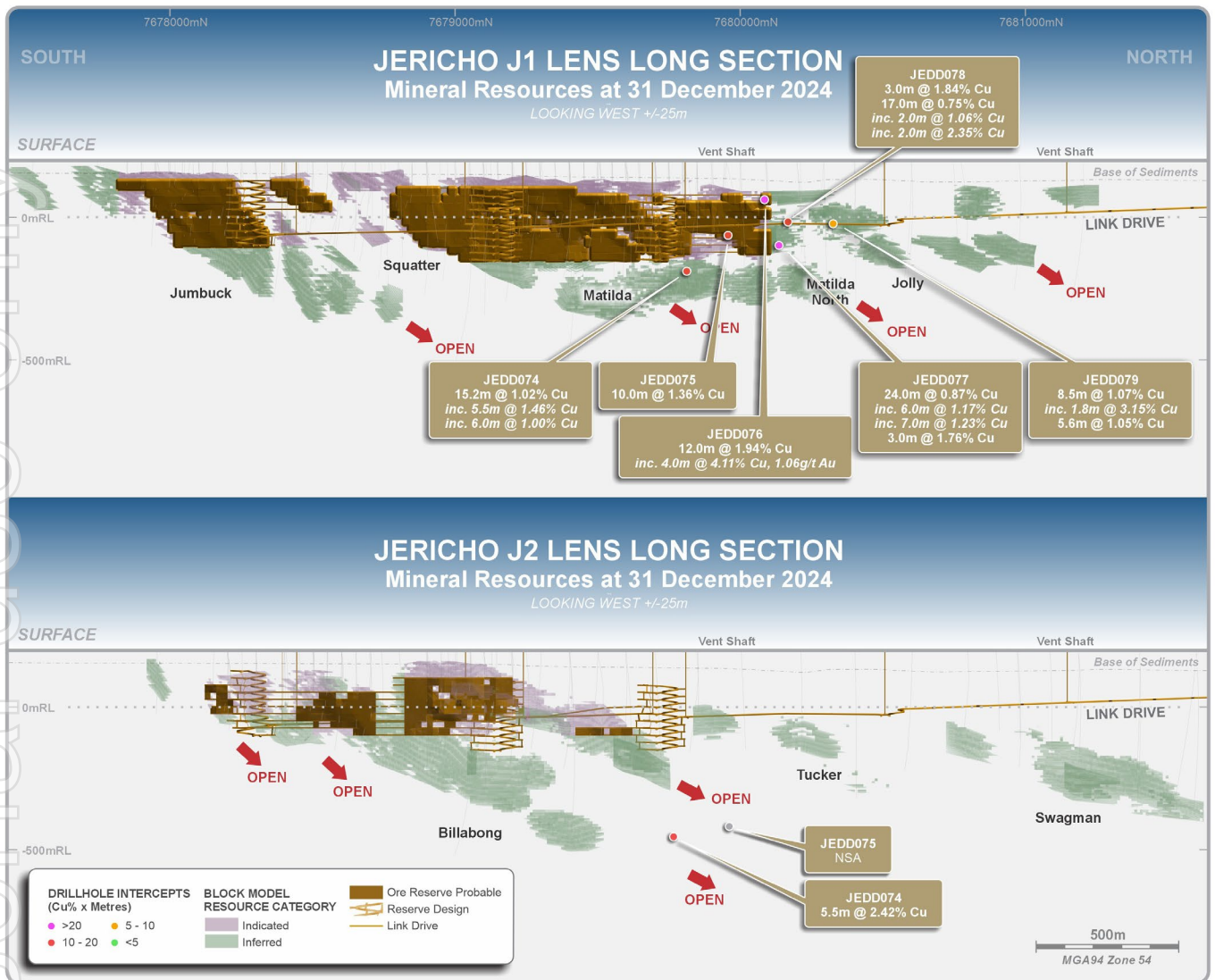
Figure 2. Jericho long sections showing location of Mineral Resource category and results of drilling
