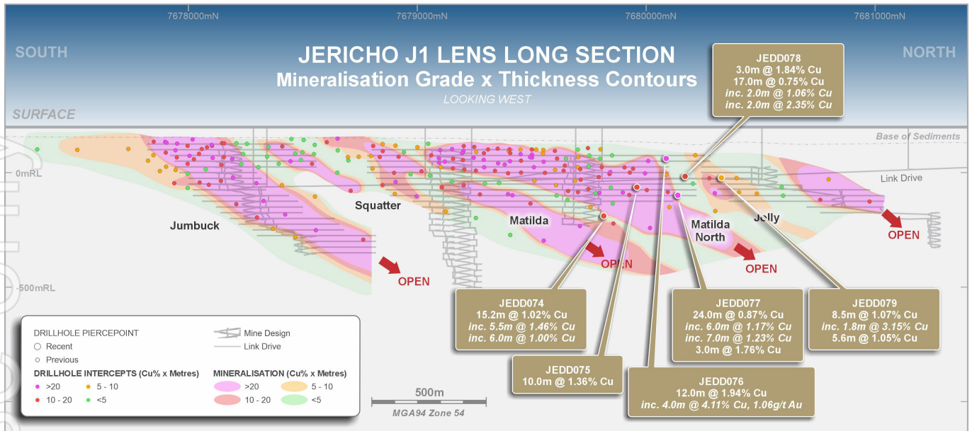
Figure 4. Jericho J1 Lens long section showing the interpreted high-grade shoots
