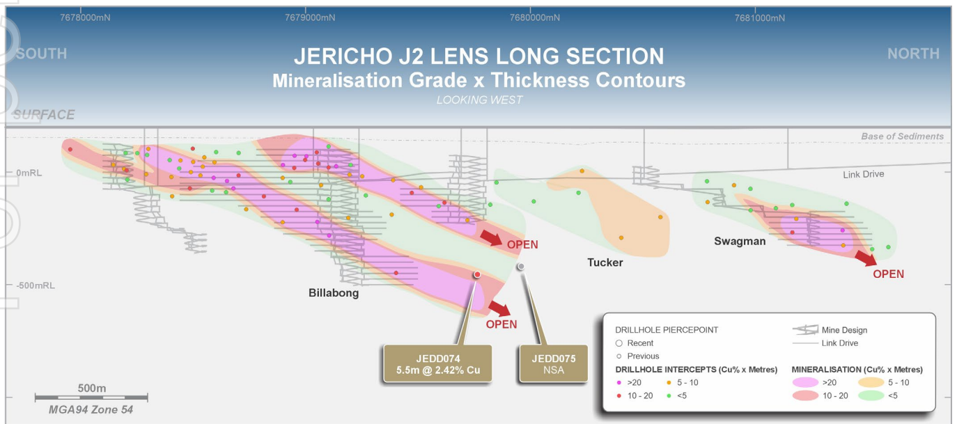
Figure 3. Jericho J2 Lens long section showing the interpreted high-grade shoots
