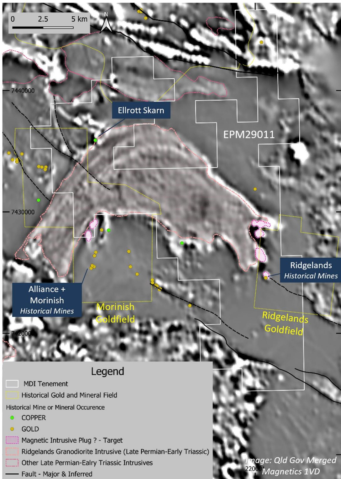
Figure 3. Regional magnetic image illustrating the relationship of the Ridgeland Goldfield, other historical mining workings, and the mapped and interpreted intrusive complex. Note white on the greyscale image corresponds to magnetic highs.
