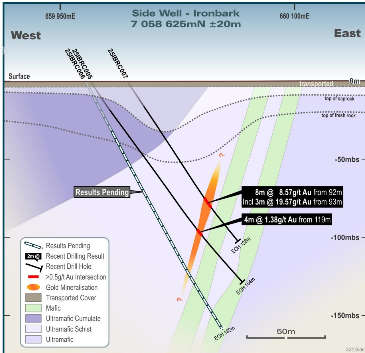
FIGURE 2: CROSS SECTION SHOWING THE RECENT DRILLING SOUTH OF IRONBARK
