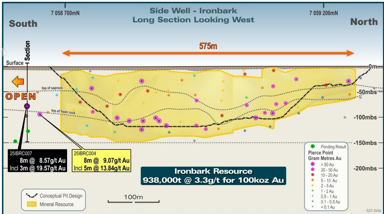
FIGURE 3: A PROJECTED LONG SECTION THROUGH IRONBARK LOOKING WEST, SHOWING THE CURRENT MRE OUTLINE, A CONCEPTUAL PIT OUTLINE AND THE RECENT RC INTERSECTIONS AT THE SOUTH END.
