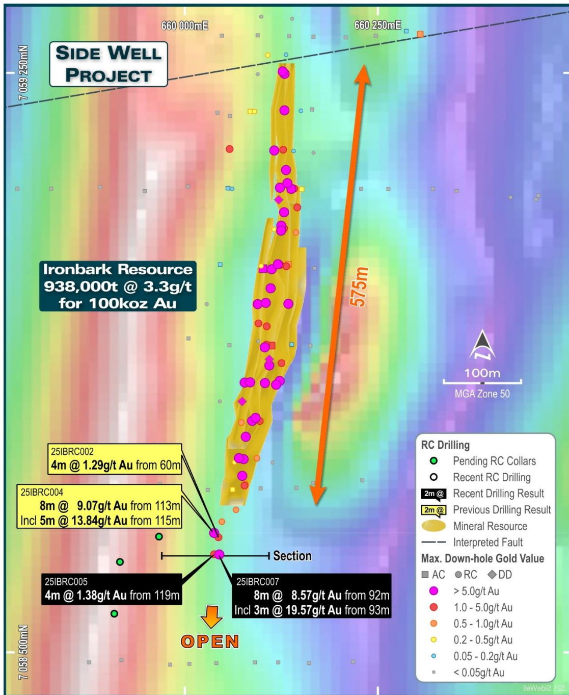
FIGURE 1: RECENT RC RESULTS AT IRONBARK. BACKGROUND IMAGE IS RTP MAGNETICS.
