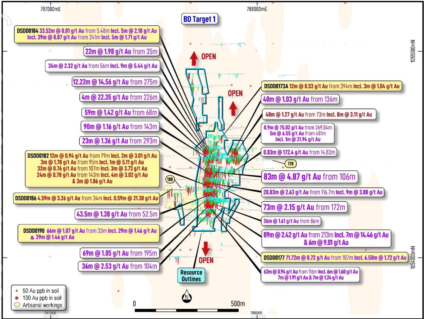
Figure 4: BD tenement plan view showing new drilling results (yellow) at BD Target 1 12
