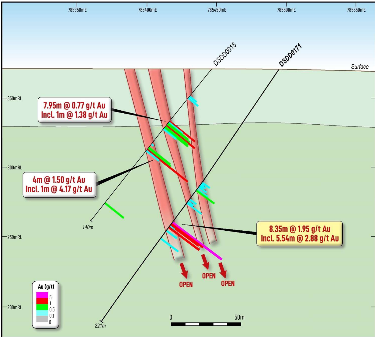
Figure 7: Cross Section looking north (+/-25m) showing new drill results DSDD0171 – BD Target 3
