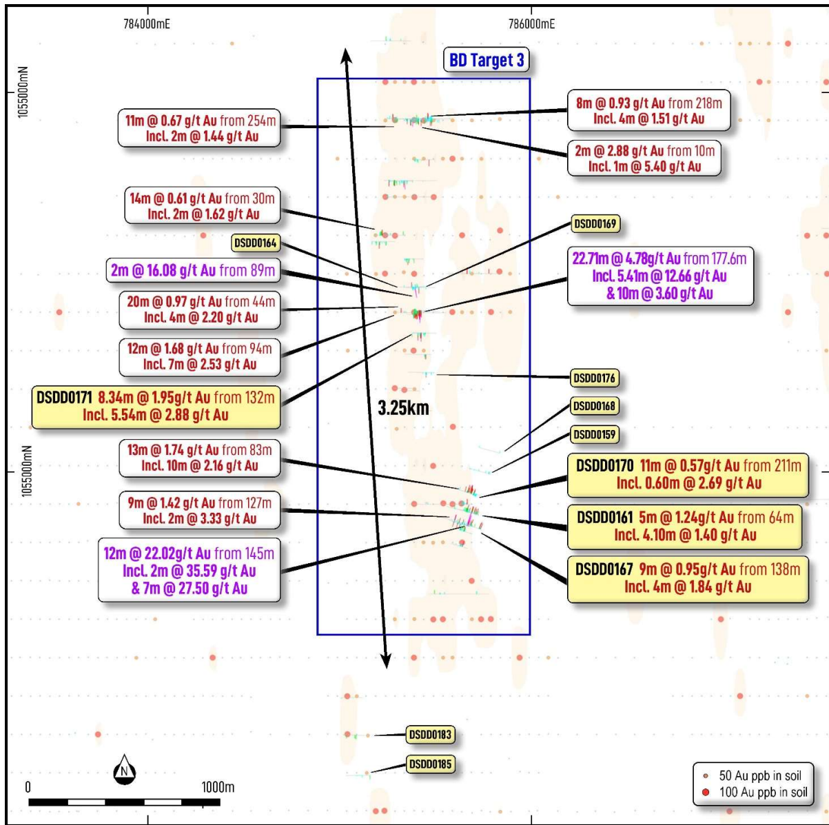
Figure 6: BD tenement plan view showing new drilling results (yellow) at BD Target 3 13
