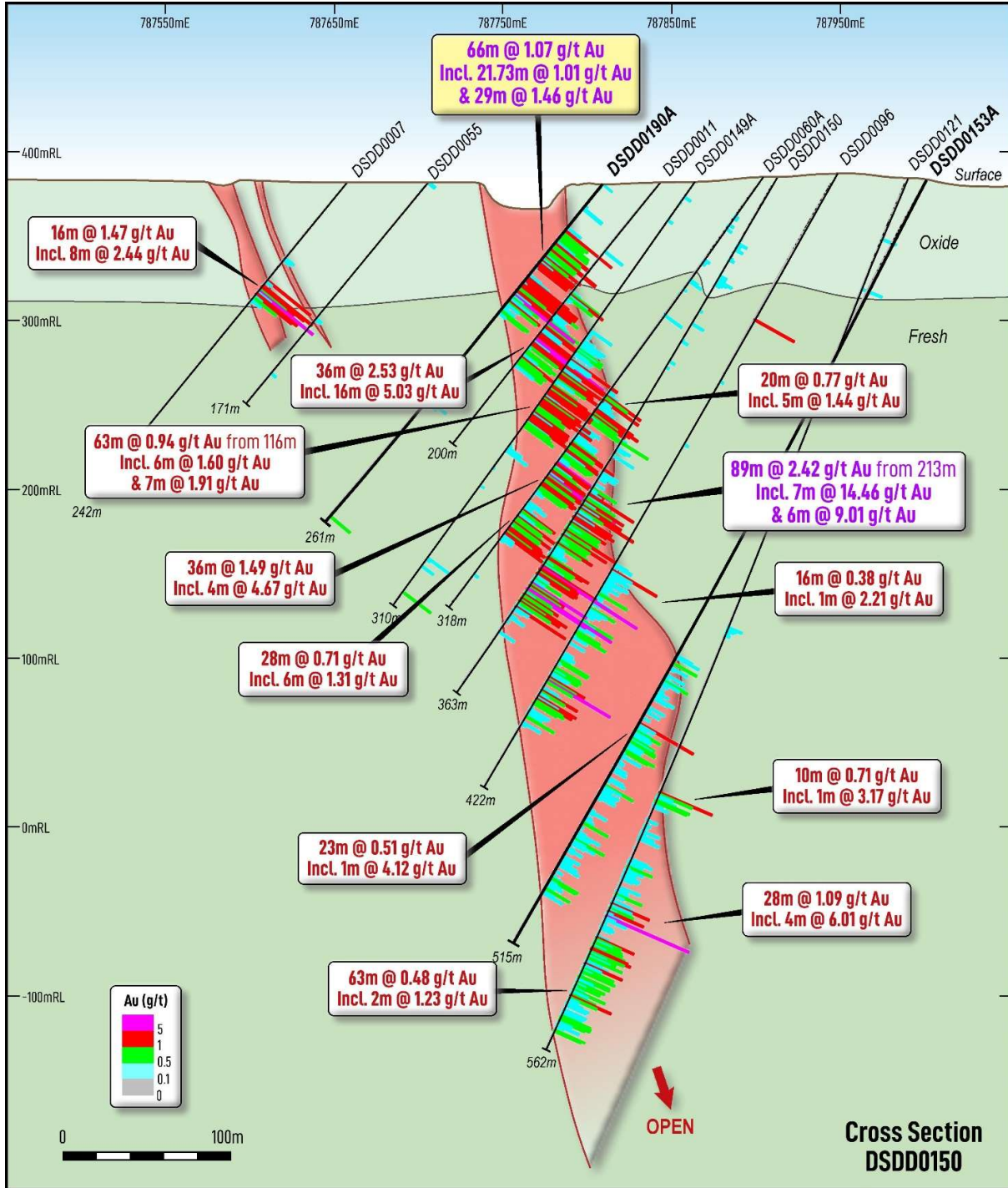
Figure 5: Cross Section looking north (+/-25m) showing new drill results DSD0190A – BD Target 1
