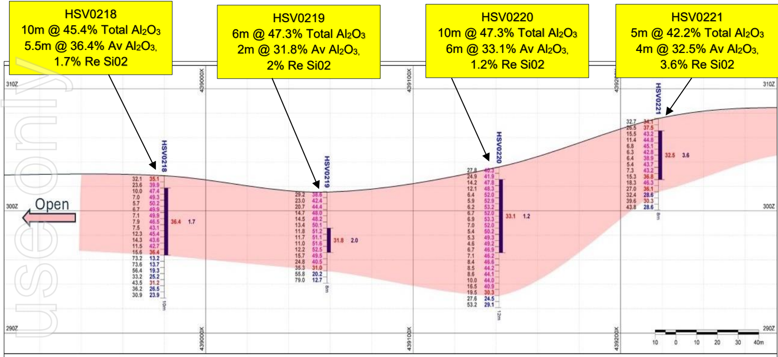
Figure 4 - Cross Section 1: 6511600N highlighting bauxite Total Al 2 O 3 % (left) & Available Al 2 O 3 %, Reactive SiO 2 % assays (Right hand - Blue column)
