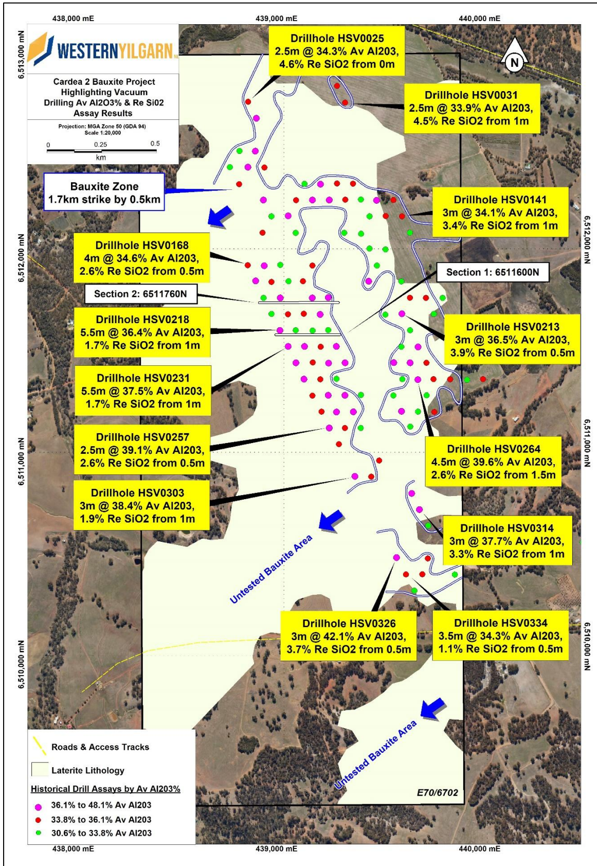
Figure 3 – Location of Bauxite Zone based on downhole Available Al 2 O 3 & Re SiO 2 Grade within E70/6702
