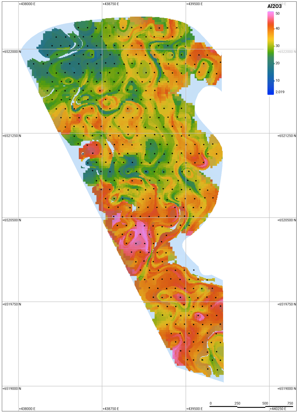
Figure 6 - Cardea 2 Block Model Plan View Showing Drillhole Total Al 2 O 3 % Assays
