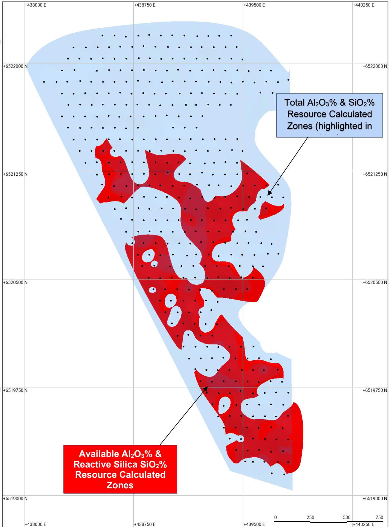
Figure 7 - Plan highlighting the various Total and Available Al 2 O 3 % over MRE Area
