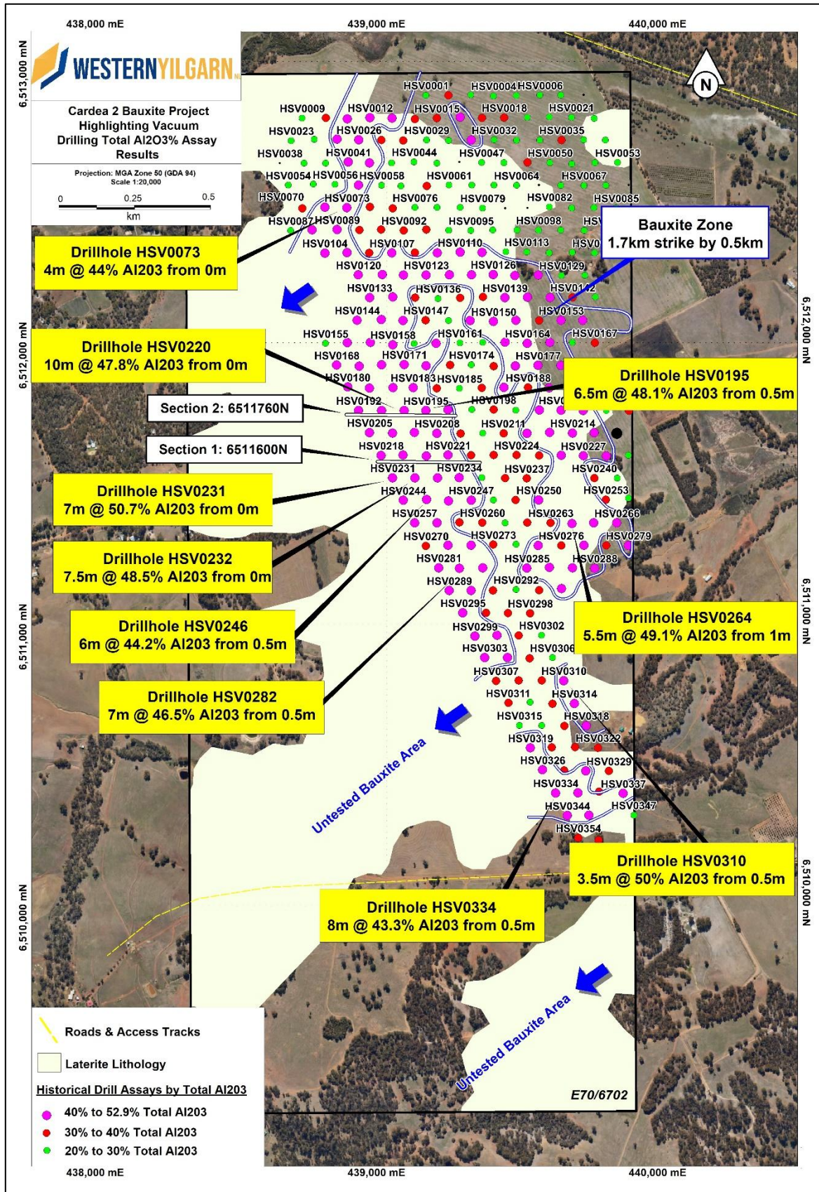
Figure 2 – Location of Bauxite Zone based on downhole Total Grade within E70/6702
