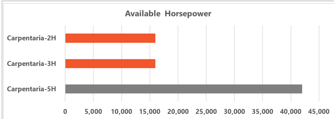
Comparison of available hydraulic horsepower between C-2H, C-3H and planned C-5H
