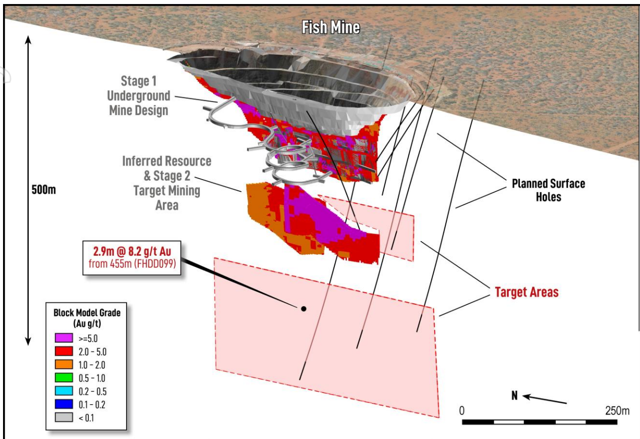
Figure 2 – Planned surface drill holes at the Fish Underground Mine
