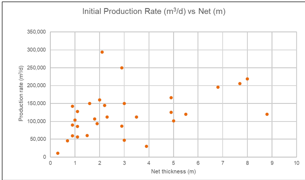
Figure 7: Hall Formation – Initial Well Production Rates vs. Net Sand Thickness
