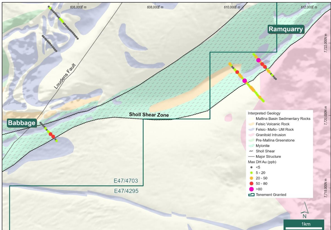
Figure 3: AC collar locations over regional geological interpretation and airborne magnetics, showing maximum downhole gold values
