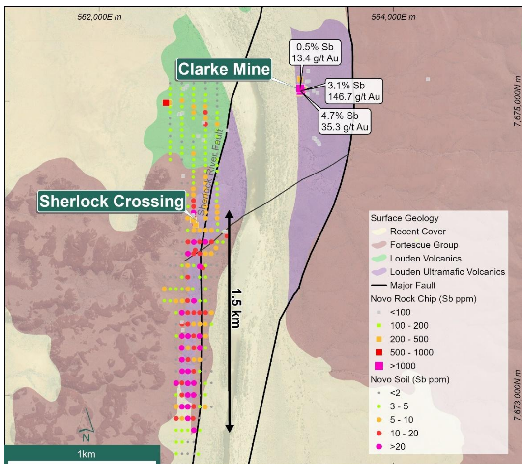
Figure 4: Sherlock Crossing, showing extended soil anomaly > 15 ppm Sb to the SW of the proposed first pass drilling area at the Clarke Mine 2
