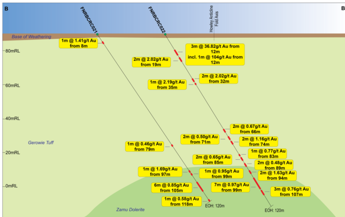
FIGURE 2: CROSS SECTION (A-A') & CROSS SECTION (B-B'): LOOKING NORTH ±20M SECTION VIEW, SHOWING INTERPRETED GEOLOGY AND SIGNIFICANT INTERSECTIONS (AU >0.30G/T). DRILLING RESULTS ARE DOWNHOLE WIDTH AND NOT TRUE WIDTH
