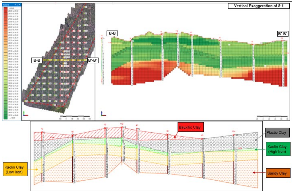
Figure 5: East-west section showing estimation of Al_2O_3 grade in the centre of the deposit
