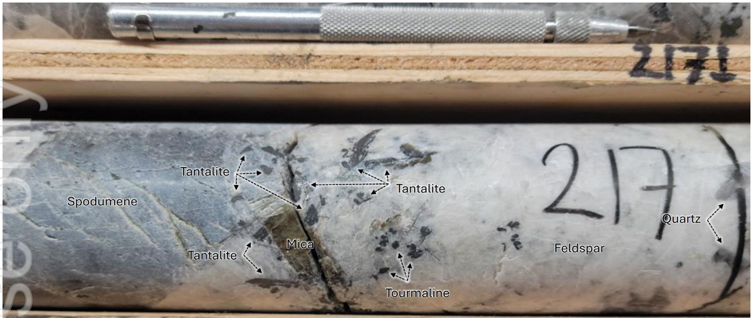
Figure 2: Very coarse-grained tantalite crystals at ~217 m depth in drill hole CV23-109 at the CV5 Pegmatite. Core grades 1,688 ppm Ta_2O_5 over 0.5 m (216.5 m to 217.0 m).
