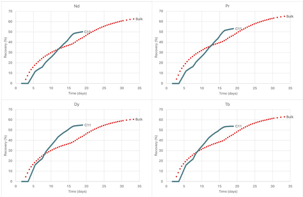
Figure 1: Recovery of Individual Magnet Rare Earth metals in small scale column leach compared to the Bulk Leach
