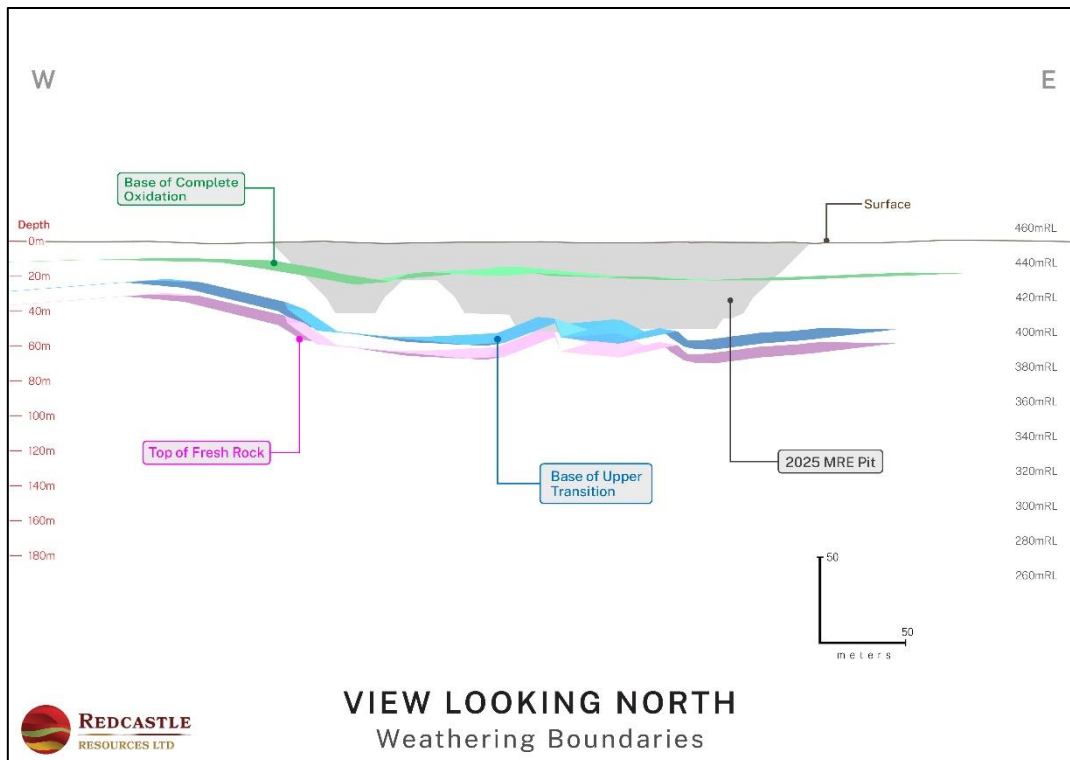
Figure 12: RR Conceptual Pit and Weathering Surfaces
