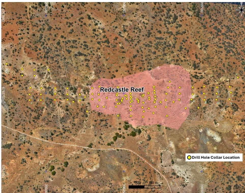
Redcastle Reef Drill Hole Collar Plan with 2025 MRE Conceptual Pit
