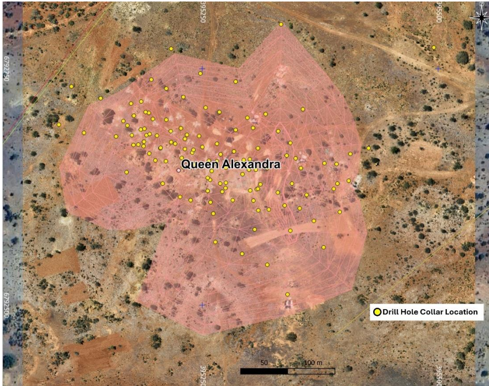
Queen Alexandra Drill Hole Collar Plan with 2025 MRE Conceptual Pit
