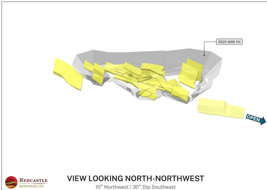
Figure 4: RR Conceptual Pit with 3D Geological Interpretation
