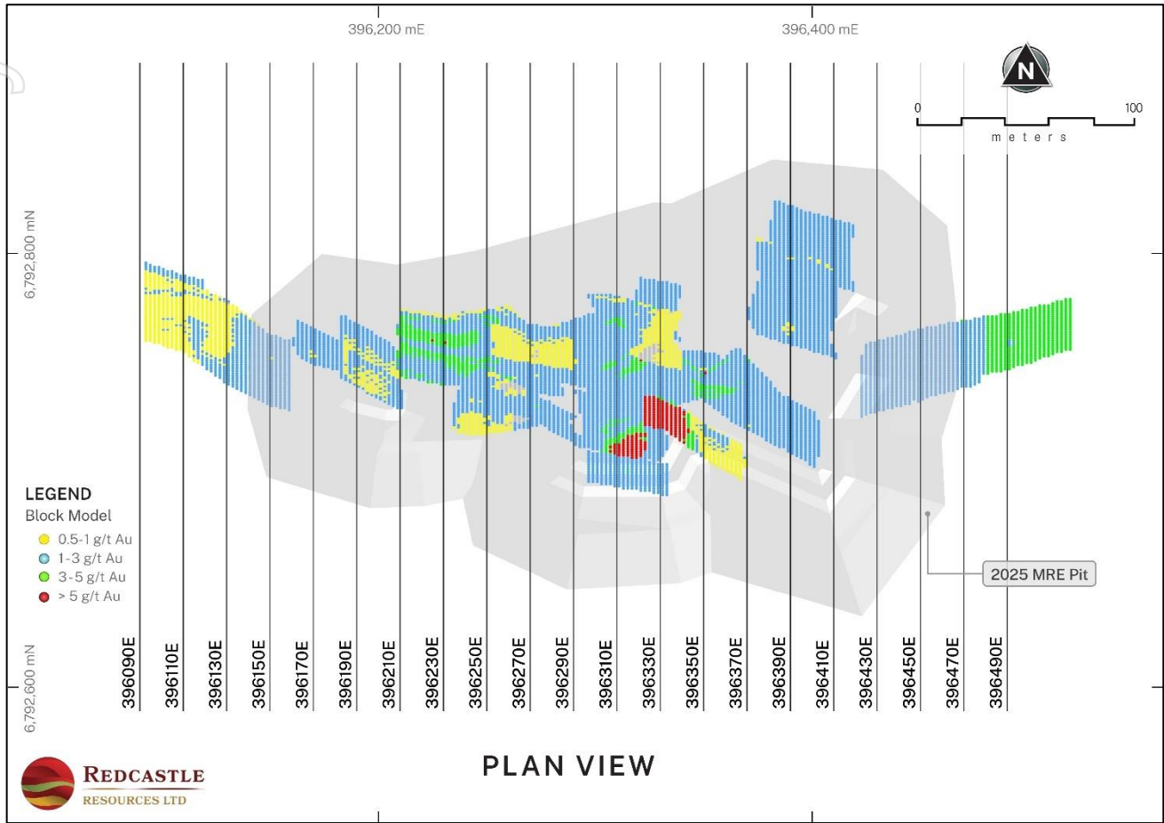
Redcastle Reef Plan Showing Section Lines
