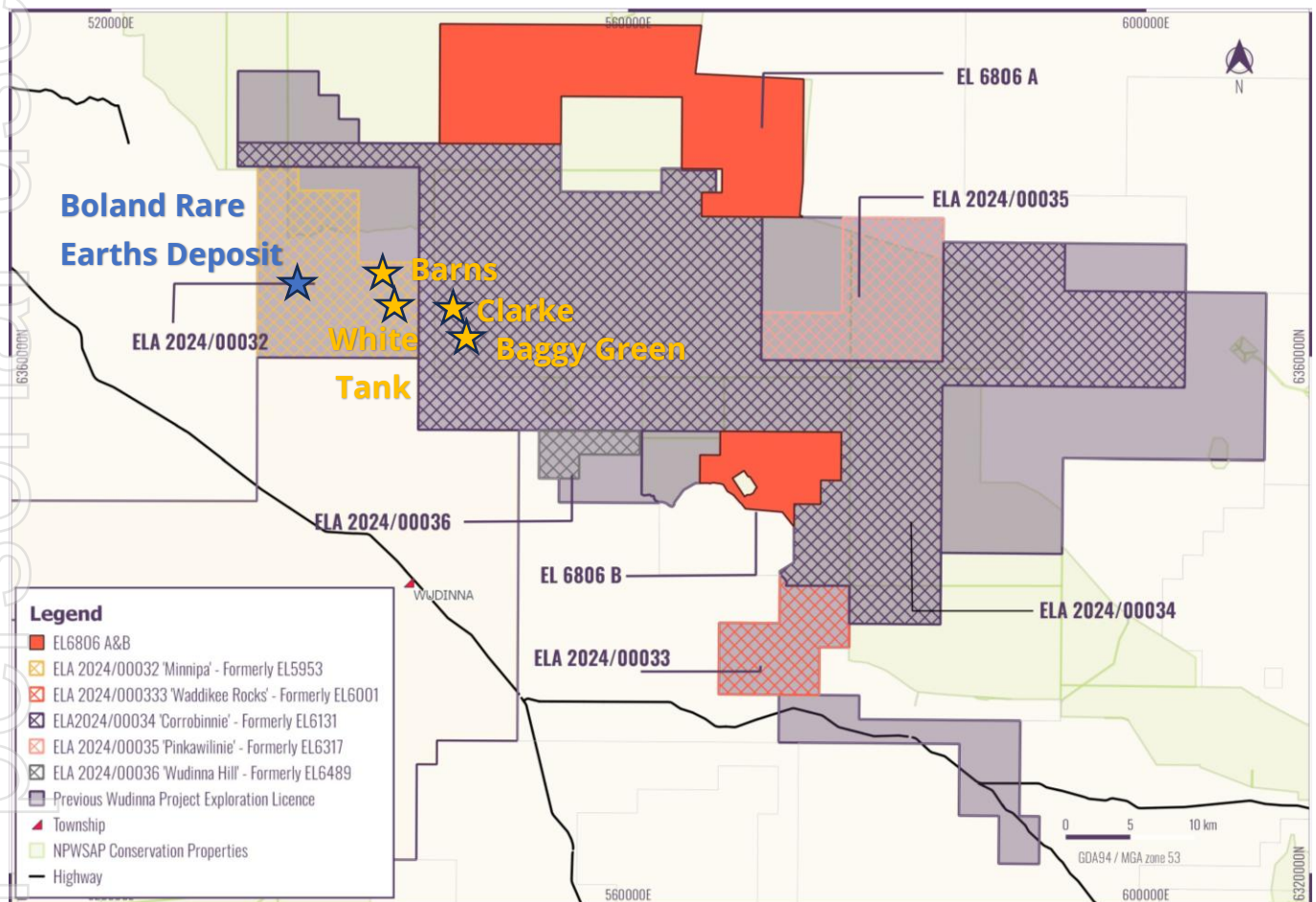
Figure 2 – Wudinna Gold Project ELAs and gold Deposits, and portions 'A' and 'B' of EL 6806
