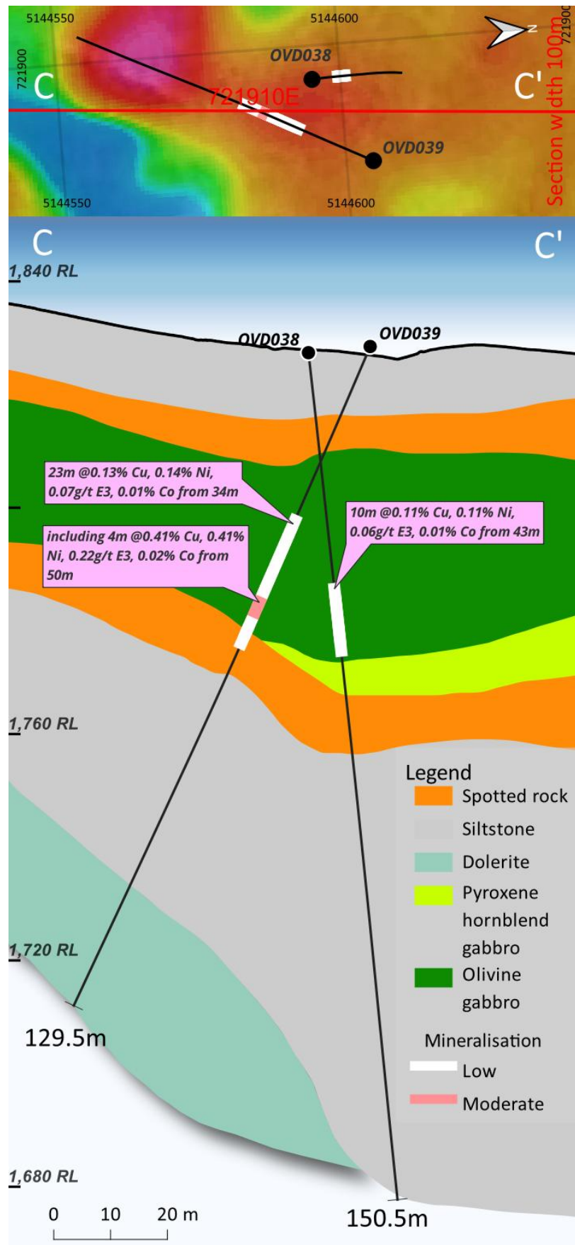
Figure 3. OVD038 and OVD039 cross-section (see Figure 1 for general location of these holes)
