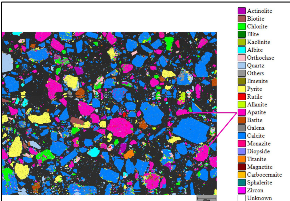
Figure 2: SEM/AMICS Mineral Image of the Polished Resin Mount. Sample ID - LnCS Composite_HG showing well liberated grains of REE-bearing apatite with monazite inclusions.
