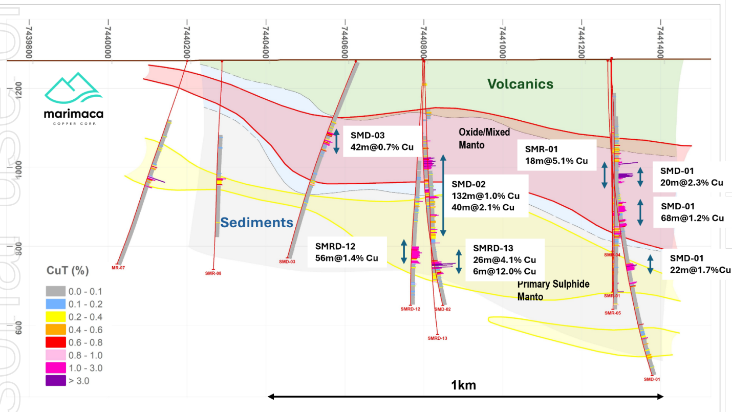
Figure 4 – Long Section Looking West – Pampa Medina
