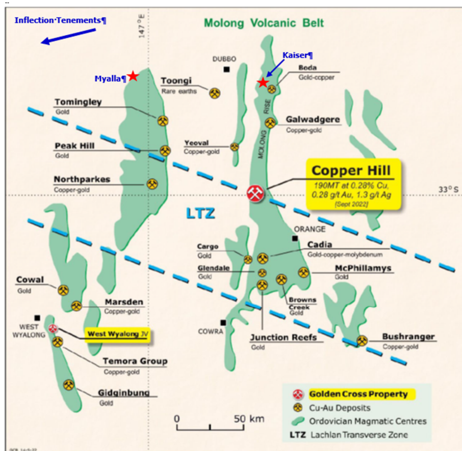
Figure 9: Copper-gold deposits of the Macquarie Arc
