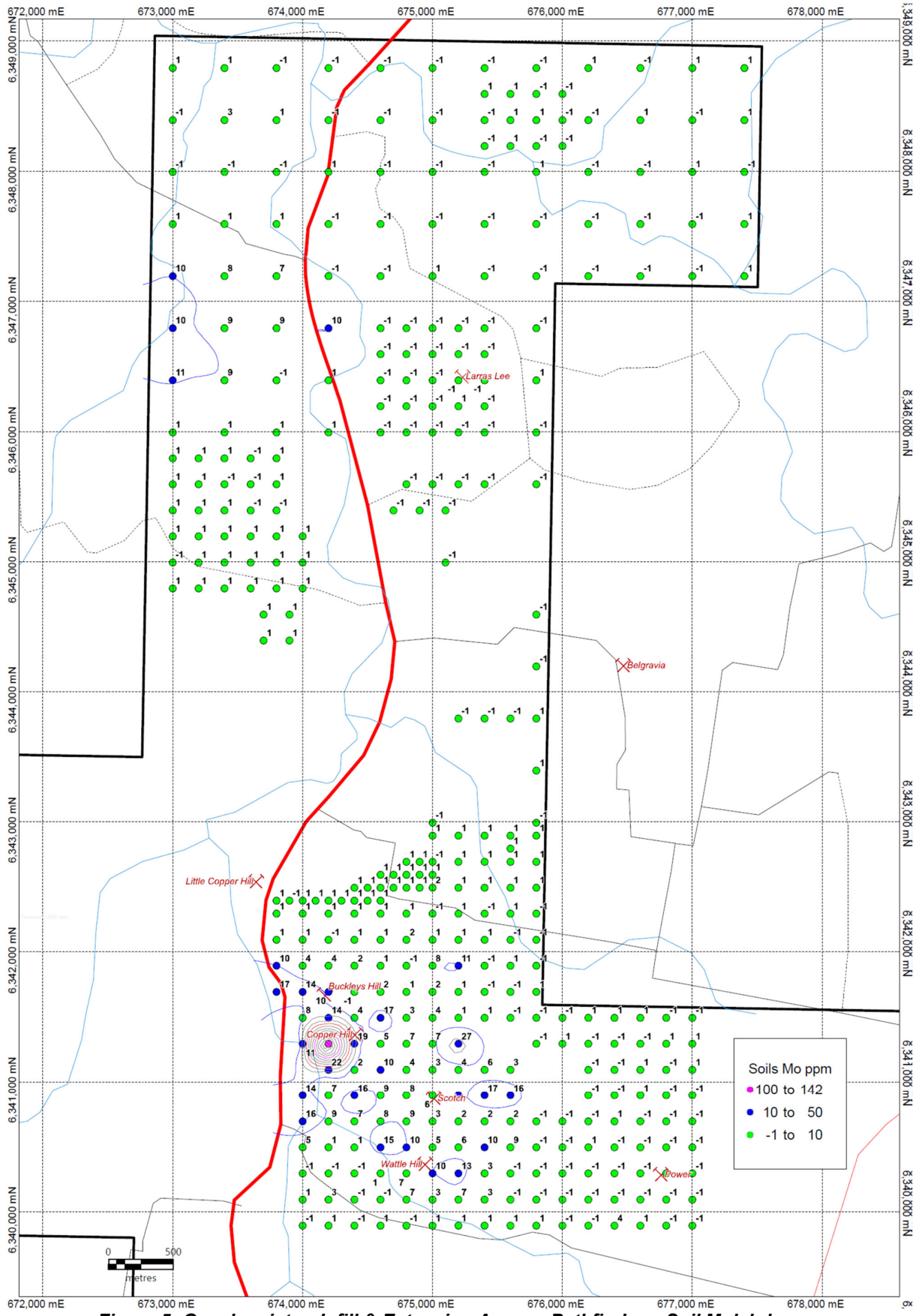
Figure 5: Geochemistry: Infill & Extension Areas – Pathfinders: Soil Molybdenum
